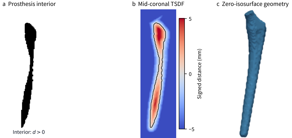
Figure 8: TSDF representation of prosthesis geometry. a , Solid femoral stem extracted from postoperative CT on a mid-coronal section. b , Continuous signed distance field on the same section; the black line marks the zero level set and distances are truncated at \pm 5 mm. c , Closed, watertight stem surface recovered from the three-dimensional zero level set.
