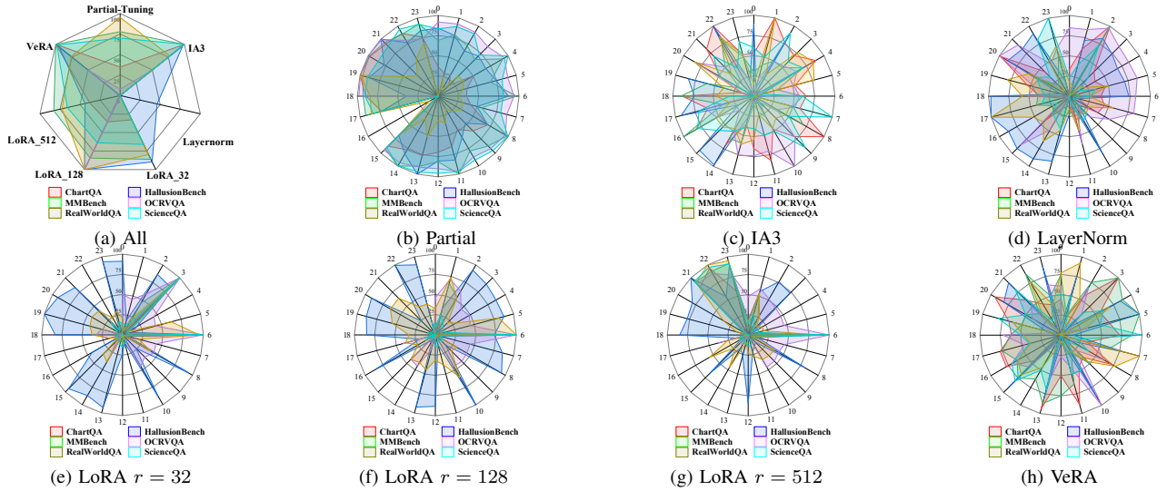
Fig. 4. Benchmark scores for all-layer tuning (a) and per-layer PEFT (b-h): Partial-T
