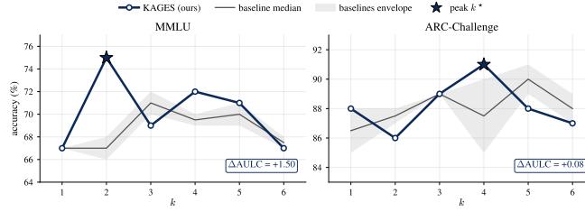
Figure 3: Accuracy curves over fused LLM count for MMLU and ARC-Challenge. The gray band spans diversity-greedy and fixed-order baselines, the gray line shows their median, and KAGES is shown in navy with stars marking its peak. The peak-then-decline pattern reproduces at the LLM layer.
