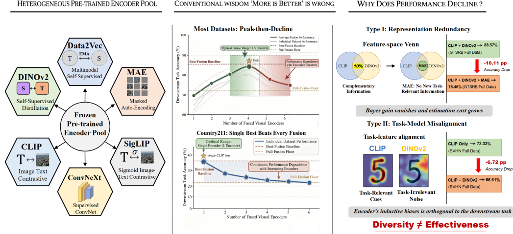
Figure 1: View-set composition in frozen foundation-model fusion. Left: a heterogeneous pool of frozen vision backbones. Middle: downstream accuracy is non-monotonic in the number of fused views, with most datasets peaking at 3 to 5 encoders and declining, while a single task-aligned encoder beats every fusion on Country211. Right: two failure modes behind the decline. Type I ( representation redundancy ): a new encoder repeats information already captured. Type II ( task-model misalignment ): a representationally distinct encoder injects task-irrelevant cues, so diversity alone is not effectiveness. The marginal-utility theory of Section 2.2 explains the shape from a single gain-cost crossing (Theorem 1); the two failure modes are formalised in supplementary App. A.3.6.
