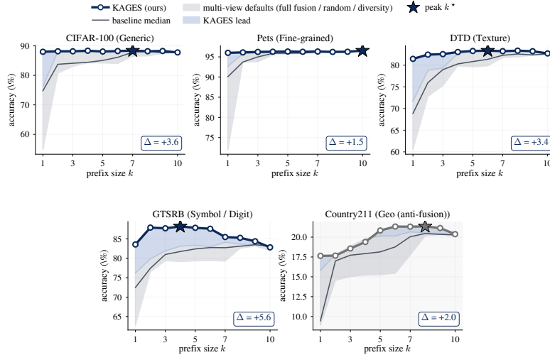
Figure 2: KAGES front-loads high-utility encoders and stays at the top of the multi-view baseline envelope (Protocol F, full data). Per-dataset prefix accuracy along each method’s ordering. KAGES (navy, star at its peak) is plotted over the gray envelope spanning the standard multi-view defaults (full fusion, random, and diversity selection), with their per- k median in gray. KAGES reaches a strong representation at small k on every regime while the defaults climb slowly, with the clearest separation on the texture and symbol tasks. Country211 is the anti-fusion regime in which CLIP alone saturates geolocation, so all methods converge.
