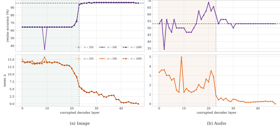
Fig. 5: Causal readout of modality information measured by single-layer corruption of the modality-token residual across depth. The top row shows classification accuracy, and the bottom row shows the mean absolute shift in the yes–no logit margin. For the image modality (left), accuracy collapses to the majority-class floor when the modality-token residual is corrupted at any layer up to the readout boundary (near layer 23; dashed vertical line), but fully recovers when corruption is applied beyond this boundary. The three image curves, corresponding to \sigma \in \{250, 500, 1000\} , all identify the same transition. The audio modality (right; \sigma = 500 ) shows a similar boundary, although the effect of corruption is weaker.
