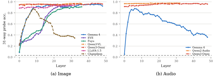
Fig. 3: Layerwise |\mathcal{C}| -way linear-probe accuracy. Encoder-free and discrete-token MLLMs develop concept decodability inside the Transformer, whereas encoder-full controls start with highly decodable representations at layer 0.
