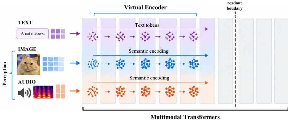
Fig. 1: Overview. When a multimodal transformer receives perceptual tokens that have not already been organized by a continuous modality encoder, it must construct a useful representation internally. In Gemma 4 12B, an early band of layers, which we call the Virtual Encoder, performs this encoding for both modalities up to a mid-depth readout boundary. There the vision representation aligns with the model’s language subspace, whereas the audio representation, though formed just as early, is not maintained downstream.
