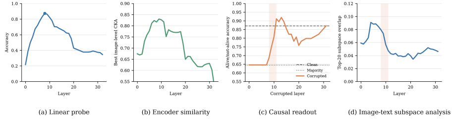
Fig. 6: Converging evidence in Chameleon. (a) Concept decodability peaks at hidden state layer 8. (b) Image-level CKA against DINOv2 is high around the same early-to-middle transition. (c) Corrupting the VQ-image-token residual collapses the alive/not-alive task to its majority floor through layer 7 and recovers across layers 8 to 11 (shaded). (d) Image-text subspace overlap follows a different trajectory from Gemma 4 12B, peaking earlier and decreasing across the causal readout window.
