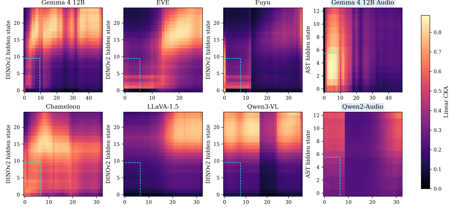
Fig. 4: Image-level CKA. The horizontal axis is the target model’s hidden state; the vertical axis is DINOv2 hidden state for vision and AST hidden state for audio. The first three columns show vision against DINOv2; the last column shows audio against AST. Dashed cyan boxes mark the first 20% of MLLM states against DINOv2 layer 0 to 9 or the first 40% of AST states.
