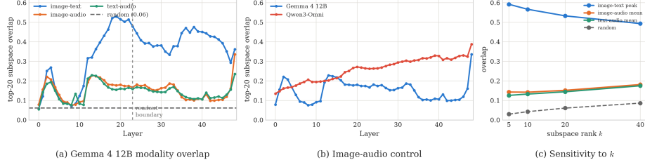
Fig. 7: Modality subspace allocation in the shared residual stream. (a) Top-20 overlap in Gemma 4 12B; the horizontal dashed line is the mean overlap of independent random 20-dimensional subspaces in the original d -dimensional space. Image-text subspace alignment is maximal near the readout transition (vertical dashed line), whereas the audio pairs remain much weaker but above chance. (b) Image-audio overlap for Gemma 4 12B and the encoder-full Qwen3-Omni control. (c) The image-text peak and layer-mean audio overlaps for k \in \{5, 10, 20, 40\} , with the corresponding random baseline.
