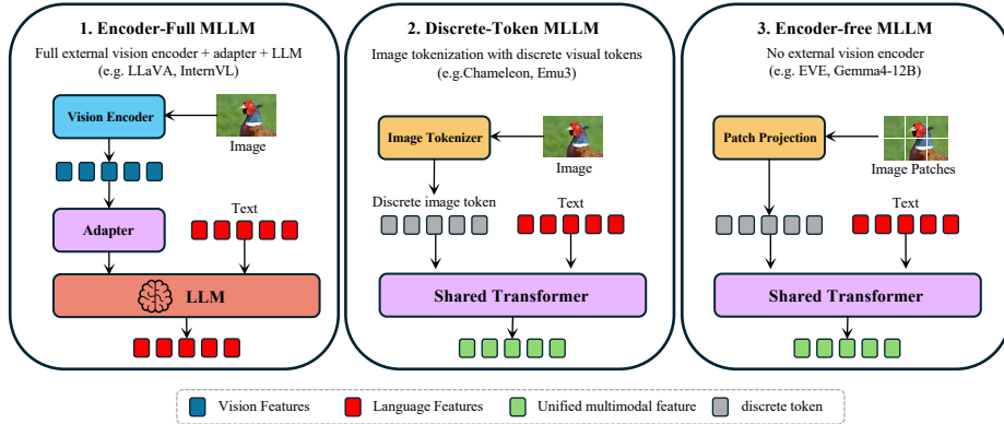
Fig. 2: Three MLLM families distinguished by the representation supplied to the multi-modal Transformer. Encoder-full MLLMs receive continuous features from a dedicated perceptual encoder. Discrete-token MLLMs receive discrete perceptual codes, while encoder-free MLLMs receive lightly projected patches or frames. We ask whether the latter two families form a Virtual Encoder inside the Transformer.
