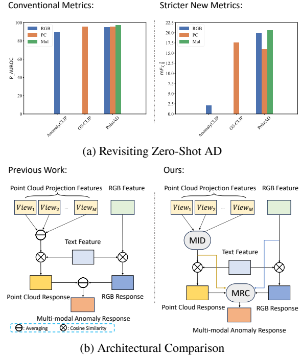
Figure 1: (a) We illustrate results using P-AUROC as a representative of conventional metrics (Bergmann et al. 2022) and mF_{1.8} as a representative of the new evaluation protocol (Zhang et al. 2026). Please zoom in for details. (b) Comparison of network architectures between our model and existing zero-shot multimodal anomaly detection methods.
