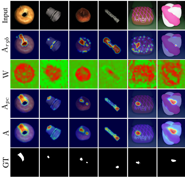
Figure 3: Visualization results of WOOPS. From top to bottom: RGB input, RGB anomaly response, RGB reliability map, point cloud anomaly response, multimodal anomaly response, and ground truth. In the reliability map, warmer red tones indicate higher confidence, whereas cooler green tones denote lower reliability. As evident, regions exhibiting erroneous RGB responses correspond to low-reliability areas, demonstrating the effectiveness of our reliability calibration.
