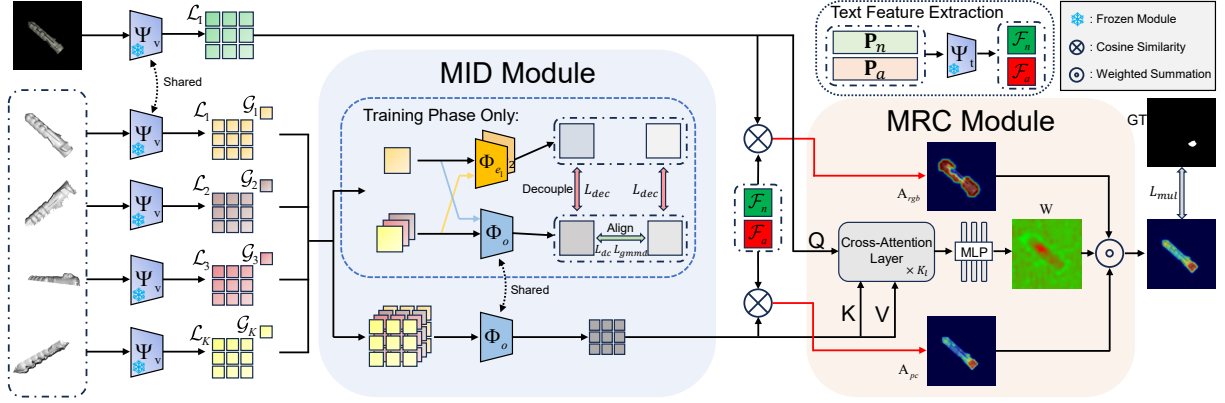
Figure 2: The pipeline of WOOPS. WOOPS employs a frozen CLIP vision encoder \Psi_v to extract RGB and point cloud features from images and multi-view projections, respectively, while utilizing a frozen CLIP text encoder \Psi_t to derive text features from learnable normal and abnormal language vectors ( \mathbf{P}_n and \mathbf{P}_a ). Anomaly responses are computed via vision-language similarity. Furthermore, we propose a Multi-view Information Decoupling (MID) module to enhance point cloud features and a Modality Reliability Calibration (MRC) module to effectively calibrate anomaly responses across modalities.
