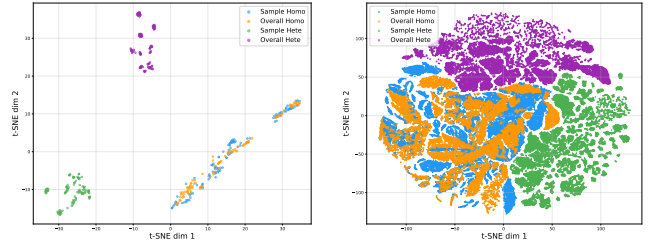
(a) Visualization of Global Feature Distributions via t-SNE (b) Visualization of Local Patch Feature Distributions via t-SNE
