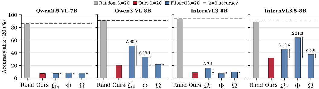
Figure 2: Causal validation of head-scoring variants on RefCOCO [5] across four VLMs [6–9]. We mask the top-20 heads detected by each variant and report visual grounding accuracy; lower accuracy indicates that the detected heads are more causally important. Ours denotes our default variant (\mathcal{Q}_s^{\text{out}}, \Phi^{\text{sum}}, \Omega^{\text{mean}}) . The \mathcal{Q}_s , \Phi , and \Omega ablations each change one component of this default design at a time, while Random masks 20 randomly selected heads. The dashed line shows the unmasked model ( k = 0 ), and \Delta denotes the accuracy gap relative to Ours .
