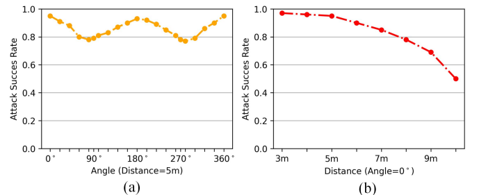
Fig. 12. Analysis of physical attack effects at (a) different angles and (b) different distances.
