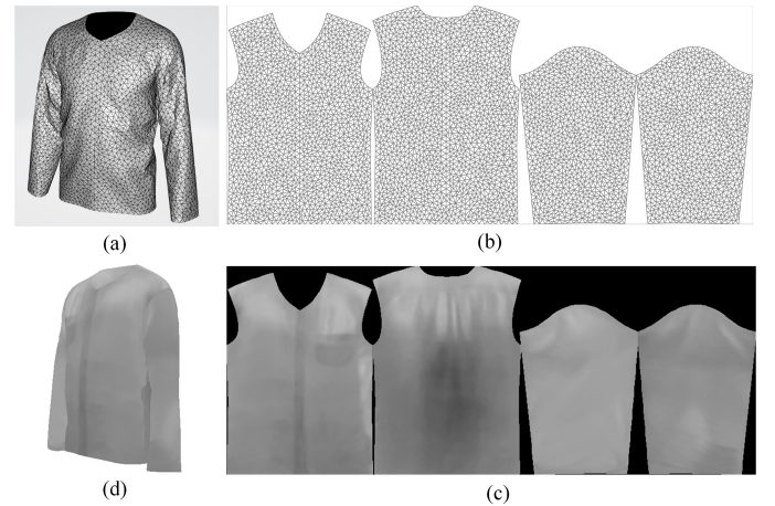
Fig. 3. Construction of 3D clothing model with real infrared characteristics. (a) 3D clothing mesh model. (b) Faces map of 3D clothing model. (c) infrared texture map of 3D clothing model. (d) Rendered 3D infrared clothing model.
