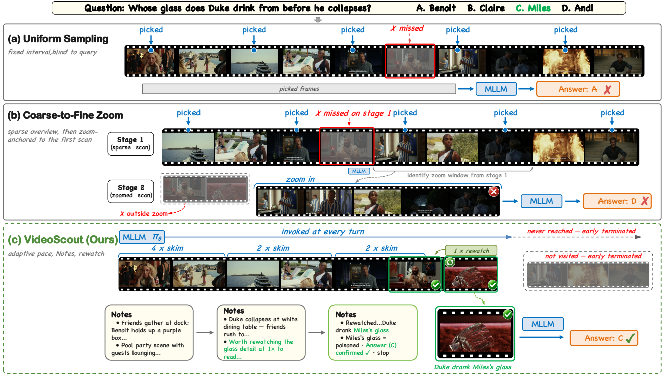
Fig. 1. VideoScout versus prior long video understanding paradigms on the same event-centric query. (a) Uniform sampling picks frames at fixed intervals and simply does not include the key frame. (b) Coarse-to-fine zoom anchors its zoom window on a sparse first-pass summary that has already missed the key frame, so the zoom window lands on the wrong interval and the evidence remains outside. (c) VideoScout consumes the video turn by turn, adapts its viewing pace over contiguous turn spans (bracketed N \times labels), maintains evolving textual Notes, and rewatches an earlier turn from the current turn when new evidence calls for it, arriving at the correct answer.
