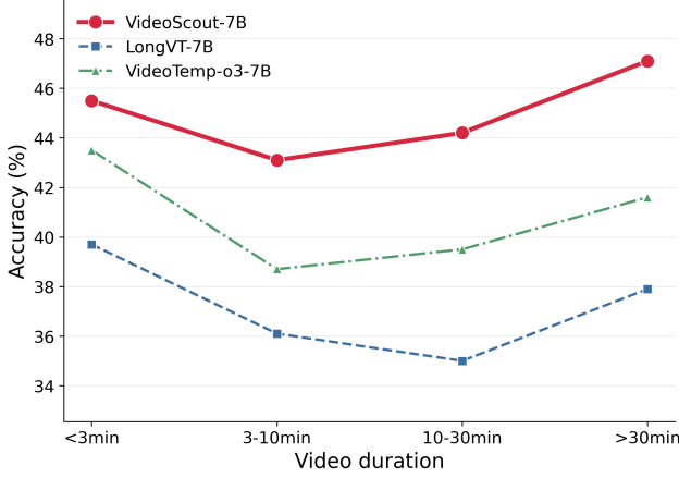
Fig. 8. Accuracy across video durations, averaged over all nine benchmarks pooled together. Each sample is assigned to a duration bucket according to its video length, and the accuracy within each bucket is reported for VideoScout and two agentic baselines.
