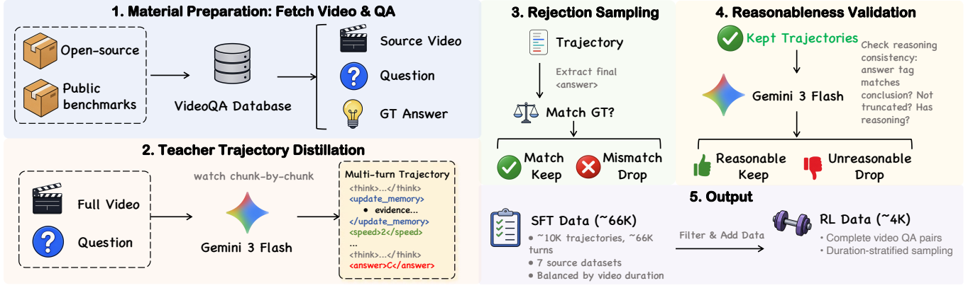
Fig. 4. The five-stage data generation pipeline of VideoScout-66K: Material Preparation, Teacher Trajectory Distillation, Rejection Sampling, Reasonableness Validation, and Output.
