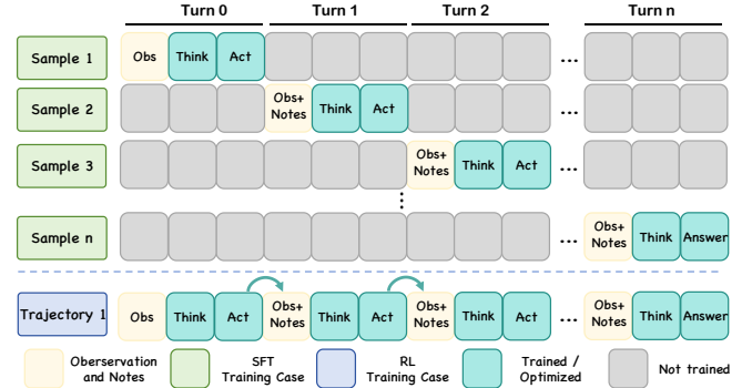
Fig. 3. Comparison between the SFT and RL training schemes. SFT optimizes individual turns independently at the turn level, where each training case corresponds to a single turn of a trajectory, whereas RL optimizes the entire multi-turn trajectory as a whole at the trajectory level.
