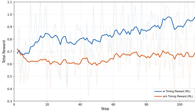
Fig. 6. Total reward curves during the RL stage with and without the timing reward. For clarity, we apply an exponential moving average with a smoothing coefficient of 0.9 to suppress step-wise noise and reveal the overall training trend.
