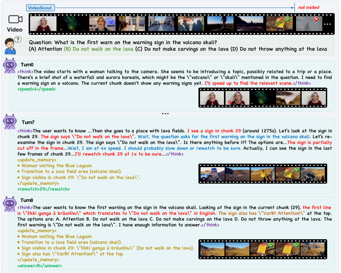
Fig. 7. A qualitative example of VideoScout on the LVBench dataset. Given a question about a long video, the agent reasons turn by turn: it adjusts the viewing speed, rewatches an earlier chunk when needed, updates its textual memory, and finally commits to an answer.
