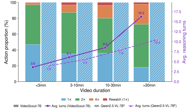
Fig. 9. Exploration behavior across video durations, aggregated over all nine benchmarks. The stacked bars show the proportion of each viewing action (1×, 2×, 4×, and rewatch), and the lines report the average number of reasoning turns per sample. Solid bars and the solid line denote VideoScout, while hatched bars and the dashed line denote the untrained agentic variant Qwen2.5-VL-7B ‡ .
