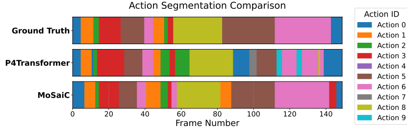
Figure 4: Qualitative comparison of frame-level action segmentation on a representative \sim 150 -frame HOI4D clip. From top to bottom, Ground Truth, the P4Transformer baseline, and MoSaiC. The horizontal axis is the frame index, and each color denotes a distinct action class, so a correct prediction requires both the color-block boundaries to align with those of Ground Truth (accurate temporal localization) and the color identity to match (correct class prediction).
