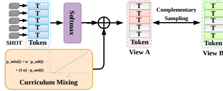
Figure 3: Structure of Curriculum Motion-Saliency Masking (CMSM). Each token’s per-frame SHOT descriptors give a motion-saliency score, which a temperature softmax converts into p_{\text{sal}} . Curriculum mixing combines p_{\text{sal}} with the uniform distribution p_{\text{uni}} under the schedule weight \alpha to obtain p_{\text{mix}} , from which View A is masked directly and View B is masked from View A’s visible tokens through complementary sampling.
