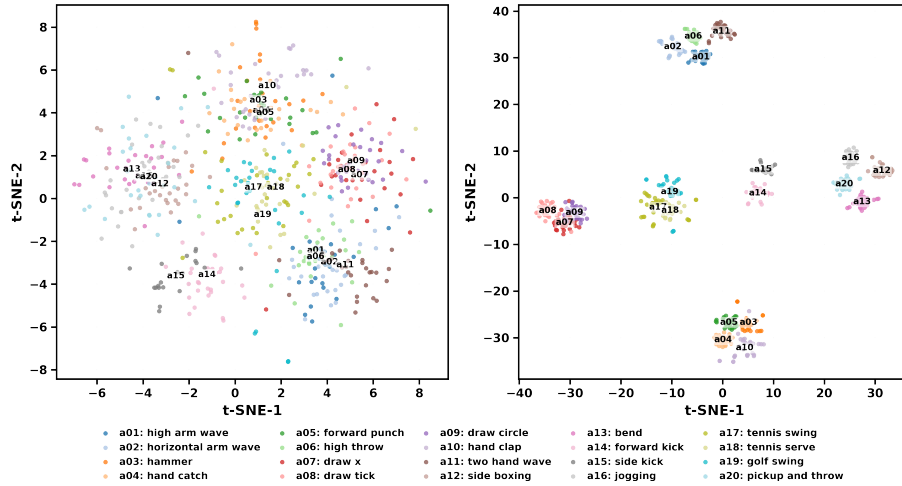
Figure 6: t-SNE visualization of the encoder features (each color denotes an action category). Left, training from scratch. Right, MoSaiC pre-training.
