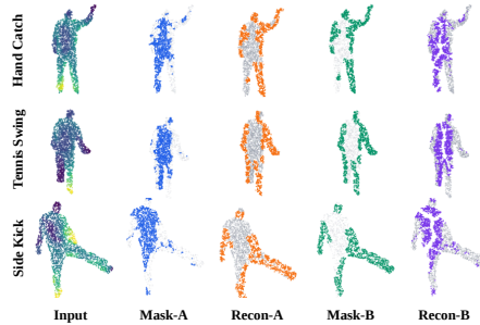
Figure 5: Qualitative visualization of complementary masking and reconstruction. For each sample we show the input, the two complementary masked views (Mask-A / Mask-B), and the corresponding reconstructions (Recon-A / Recon-B).
