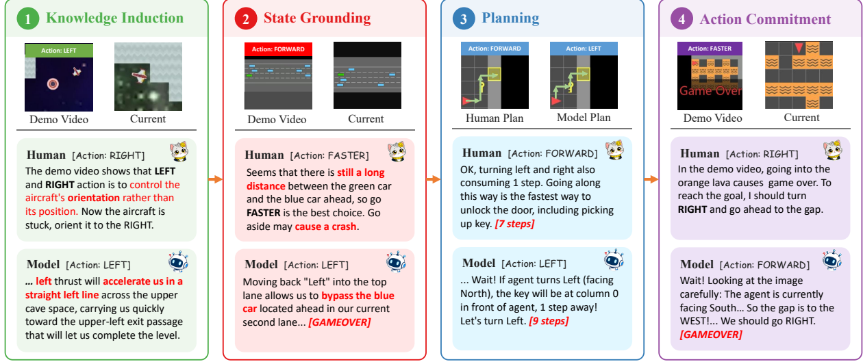
Figure 3 Representative failures across the four-stage decision-making process. Each panel contrasts the human decision with the model response at the corresponding deficient stage.
