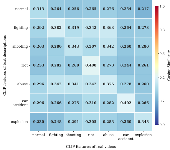
Figure 4. Similarity Matrix of CLIP Cross-Modal Features: Text Descriptions vs. Real Videos from XD-Violence dataset.
