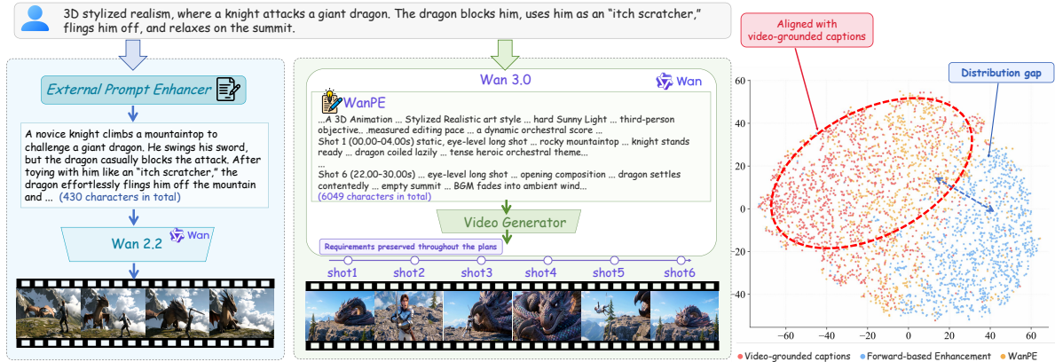
Figure 1 Left: Earlier models use optional prompt expansions, while modern video generators can process longer contexts and follow complex instructions. Right: t-SNE shows WanPE outputs align closely with video-grounded captions, while forward-based enhancement exhibits a distribution gap.
