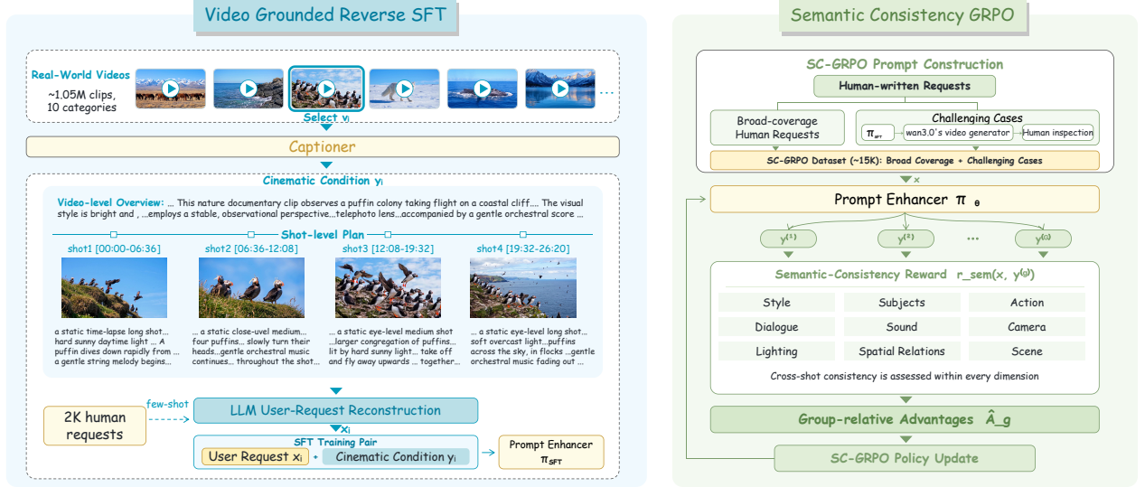
Figure 2 WanPE training pipeline. Video-grounded reverse SFT and semantic-consistency GRPO.
