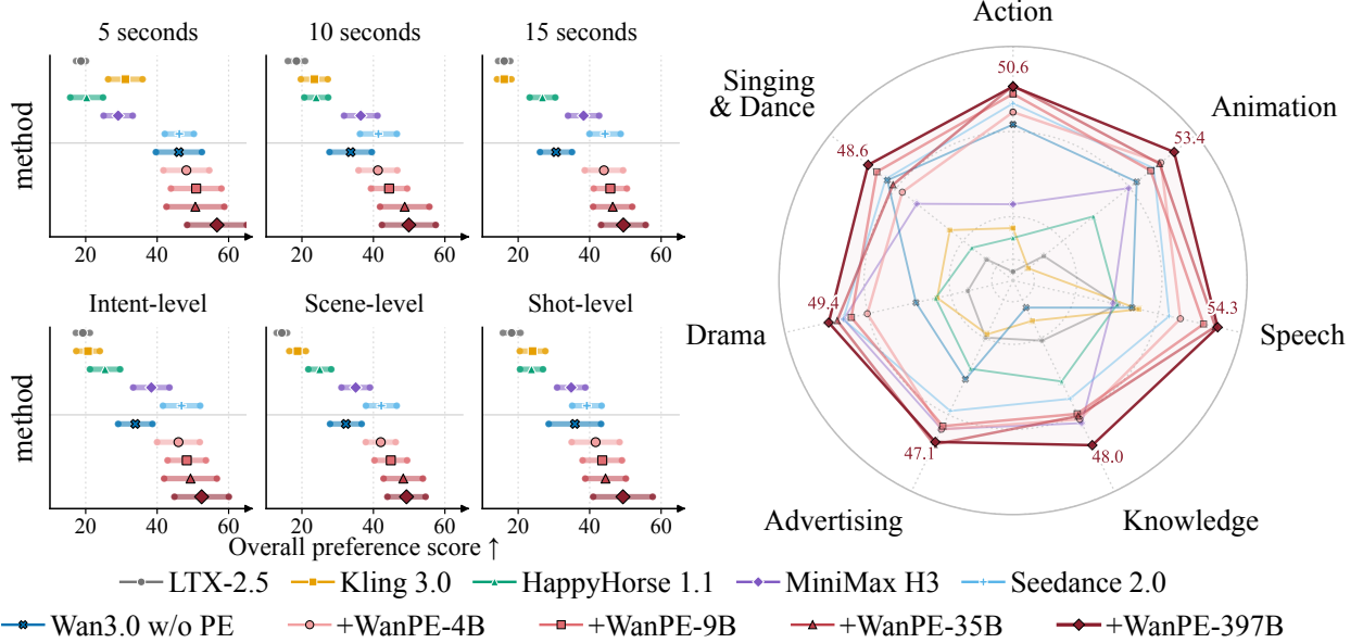
Figure 3 Fine-grained expert evaluation on the 5–15 seconds subset of WanPEval. Left: Preference scores across generation durations and request-granularity levels. Markers denote S , and horizontal intervals span [S_{\text{lower}}, S_{\text{upper}}] . Right: Preference scores S across seven content categories.
