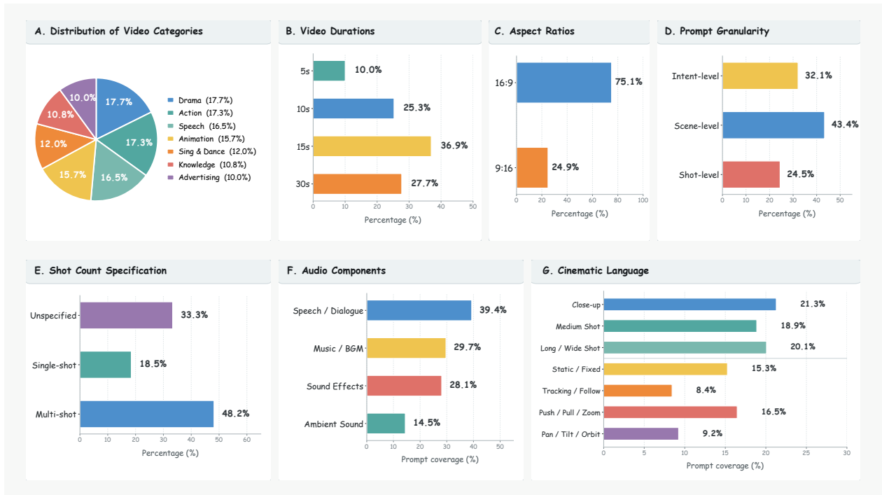
Figure 5 Distribution of the 249 requests in WanPEval. The panels report video category, target duration, aspect ratio, prompt granularity, shot-count specification, audio components, and cinematic language.
