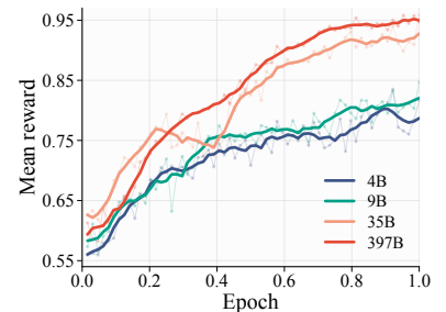
Figure 4 Mean reward during SC-GRPO training at four scales.
