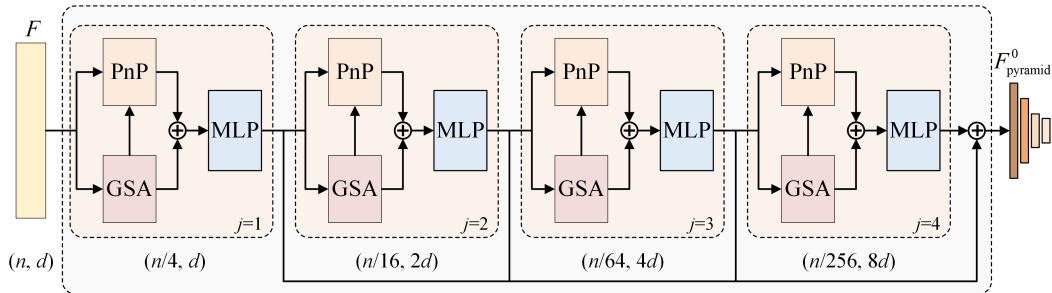
Figure 2: The structure of the fine-grained feature extraction block.
