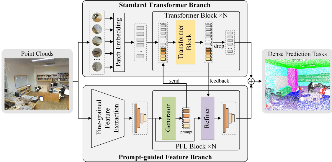
Figure 1: Overall architecture of PCT-Prompt.
