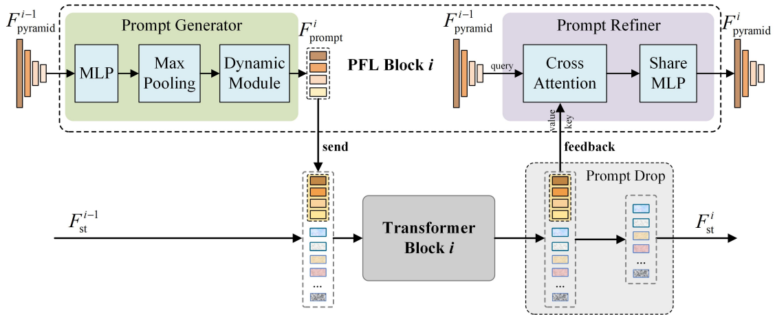
Figure 3: The structure of the prompt-refined feature learning block.
