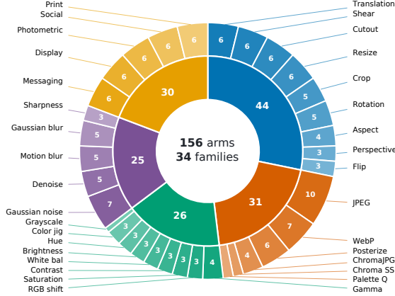
Fig. 2. Composition of the 156-arm benchmark across 34 attack families. Inner sectors: geometry (44), photometric/color (26), compression/quantization (31), filtering/restoration/noise (25), and compound (30). Outer sectors show severity-arm counts.
