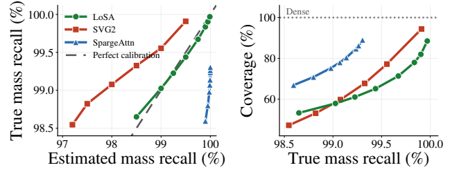
Figure 3: LoSA achieves more accurate and efficient attention-mass estimation in the near-lossless regime. The left panel plots estimated against true retained-mass recall as each method’s fidelity setting is varied. The pattern constructed by LoSA at t_0 remains close to perfect calibration, whereas the per-step estimates used by SVG2 and SpargeAttn are miscalibrated. The right panel shows the coverage required to achieve each true recall. In the near-lossless regime at or above 99% recall, LoSA consistently requires less coverage than both SVG2 and SpargeAttn.
