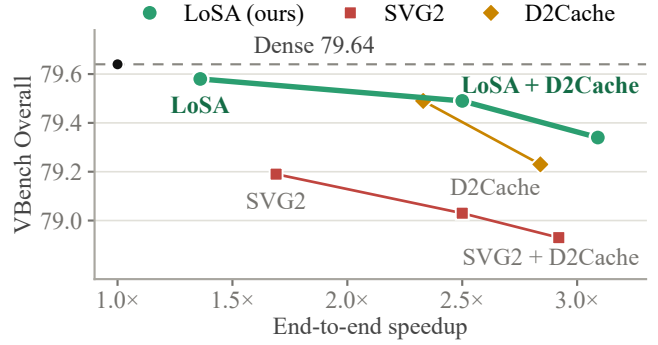
Figure 1: Speed-quality trade-off on Wan2.1-1.3B. Each point reports VBench Overall versus end-to-end speedup. LoSA and its cached variants form the entire Pareto frontier: every baseline configuration is matched or dominated by a LoSA configuration, showing that near-lossless sparse attention preserves quality better than aggressive sparsity or cache-only acceleration.
