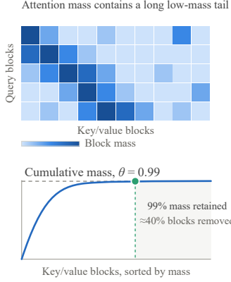
Figure 4: Overview of LoSA. Left: video diffusion attention contains a low-mass tail, allowing approximately 40% of the block area to be removed while retaining approximately 99% of the attention mass. Right: after a dense warm-up, LoSA measures exact block masses at t_0 and constructs the mask \Omega by retaining, for each layer, head, and query block, the smallest prefix whose cumulative mass reaches \theta . The same frozen mask is reused at all remaining steps, while Q/K/V and attention weights are recomputed from the current hidden states. Bottom: with optional feature caching, the cache selects which steps are computed, while LoSA accelerates self-attention within every computed step.
