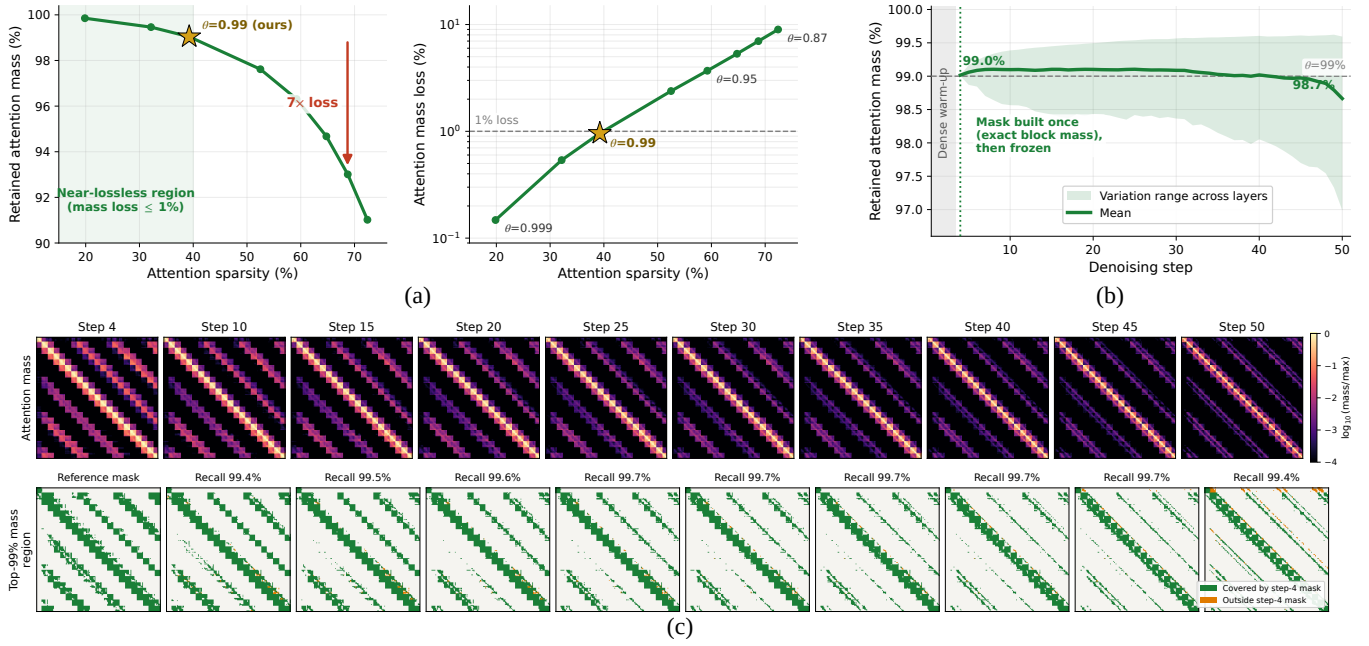
Figure 2: Empirical motivation for near-lossless sparse attention. (a) Retained attention mass versus attention sparsity (left) and the corresponding mass loss under different thresholds \theta (right). About 40% of the block area can be removed with only 1% mass loss, while further sparsity becomes disproportionately expensive. (b) Retained mass of a frozen 99%-mass pattern across denoising steps. The pattern is constructed once after the dense warm-up and keeps its recall close to 99% for the rest of the trajectory. (c) Attention maps of one head across denoising steps (top, log scale) and each step’s top-99%-mass region (bottom), colored by whether it is covered by the mask built at t_0 = 3 ; the number above each panel is the covered fraction. The high-mass region stays inside the early mask throughout denoising.
