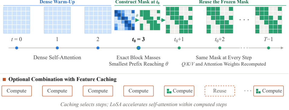
Figure 4: Overview of LoSA. Left: video diffusion attention contains a low-mass tail, allowing approximately 40% of the block area to be removed while retaining approximately 99% of the attention mass. Right: after a dense warm-up, LoSA measures exact block masses at t_0 and constructs the mask \Omega by retaining, for each layer, head, and query block, the smallest prefix whose cumulative mass reaches \theta . The same frozen mask is reused at all remaining steps, while Q/K/V and attention weights are recomputed from the current hidden states. Bottom: with optional feature caching, the cache selects which steps are computed, while LoSA accelerates self-attention within every computed step.
