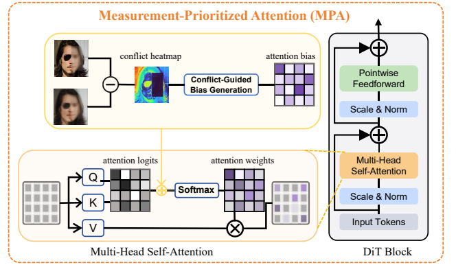
Figure 3: Overview of Measurement-Prioritized Attention (MPA). MPA summarizes prior-data conflicts as a conflict heatmap and converts it into an image-token attention bias within the DiT backbone, strengthening measurement guidance in weakly constrained regions.
