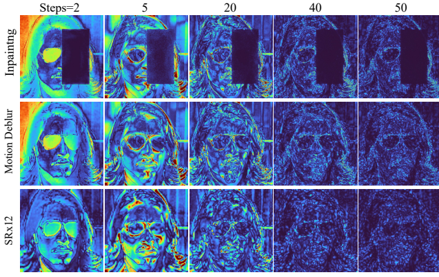
Figure 4: Data-consistency conflict heatmaps over the restoration trajectory for inpainting, motion deblurring, and \times 12 super-resolution. Brighter values indicate larger corrections between the prior and data-consistent estimates.
