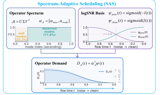
Figure 2: Overview of Spectrum-Adaptive Scheduling (SAS). SAS combines the operator spectrum and logSNR-derived temporal bases into an operator demand, which is used to distribute the finite NFE budget over flow time.
