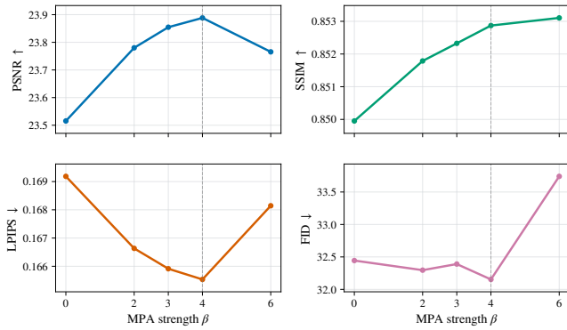
Figure 8: MPA bias-strength sensitivity with the correct heatmap on 100 FFHQ box-inpainting images using FLAIR and Global SAS with \lambda = 1 . The four panels report PSNR, SSIM, LPIPS, and FID over \beta \in \{0, 2, 3, 4, 6\} ; \beta = 0 is the no-MPA endpoint.
