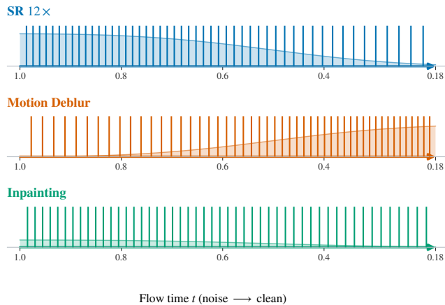
Figure 7: Global SAS schedules for SR 12\times , motion deblurring, and inpainting. Each vertical mark denotes one of the 50 solver times; colors distinguish the degradation operators, and the translucent profile shows the normalized local density of the displayed times. Flow time proceeds from noise to clean.
