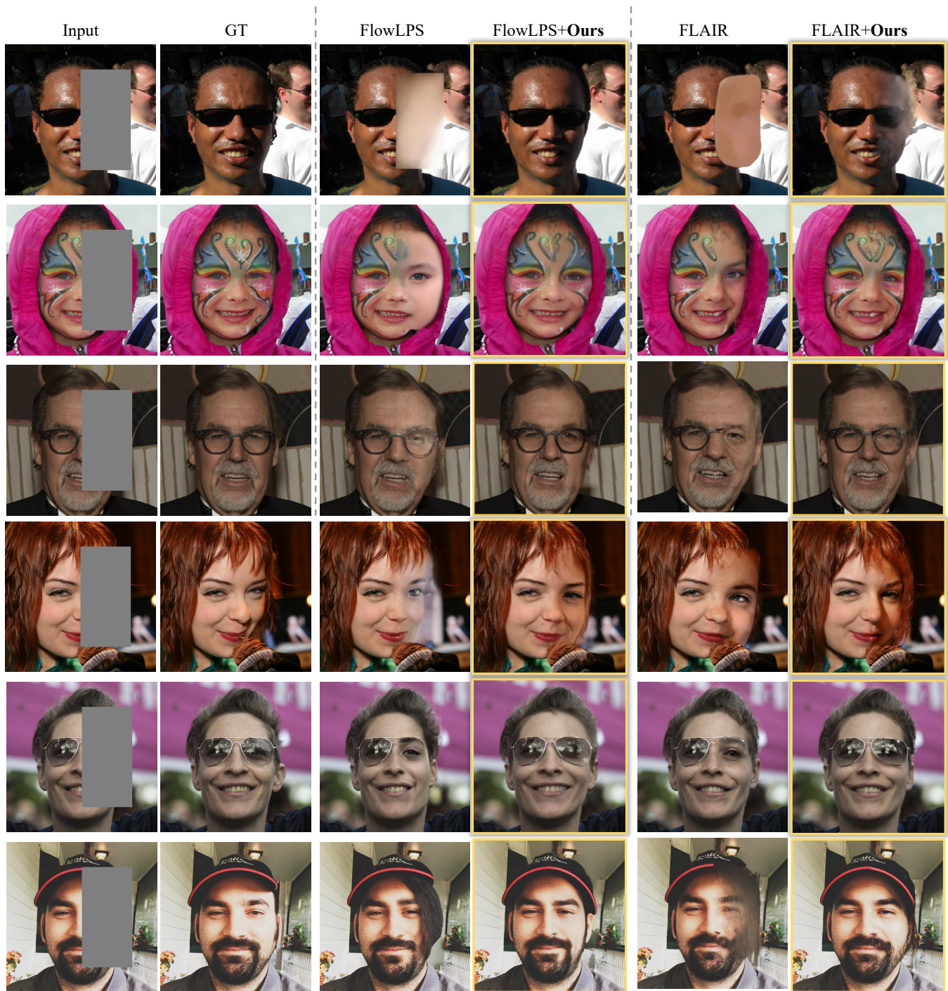
Figure 10: Additional qualitative results on FFHQ box inpainting. Under the same observations, seeds, and NFE budget, the proposed components more consistently preserve instance-specific semantic and structural cues across the masked boundary, reinforcing the inpainting observations in the main paper.
