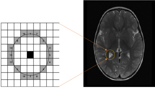
Fig. 2. Schematic diagram of the extraction of FAST feature points.
