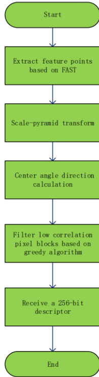
Fig. 4. ORB feature extraction and the matching flowchart.
