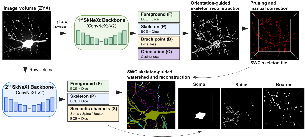
Figure 1: Overview of the SkNeXt framework.
