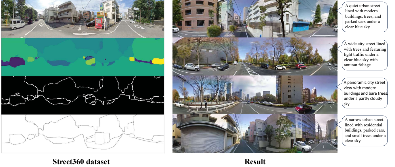
Fig. 1. Representative samples and structure prompts from the proposed Street360 dataset are shown on the left, and representative results generated by StreetDiff are shown on the right. The examples on the two sides are independently selected to illustrate the dataset characteristics and the model's generation ability.
