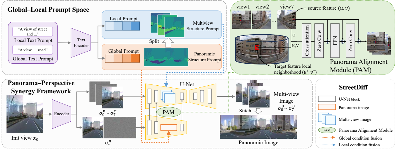
Fig. 2. The pipeline of StreetDiff. The top is the Global-Local Prompt Space, including local and global text prompts, and the corresponding structure prompts. The global text is composed by concatenating the local texts, while the multi-view structure prompt is derived by segmenting the panoramic structure prompt. The bottom is a Panorama-Perspective Synergy Framework: a panoramic generation and a multi-view generation module. The global and local conditions are inserted into the panorama and multi-view generation branches, respectively.
