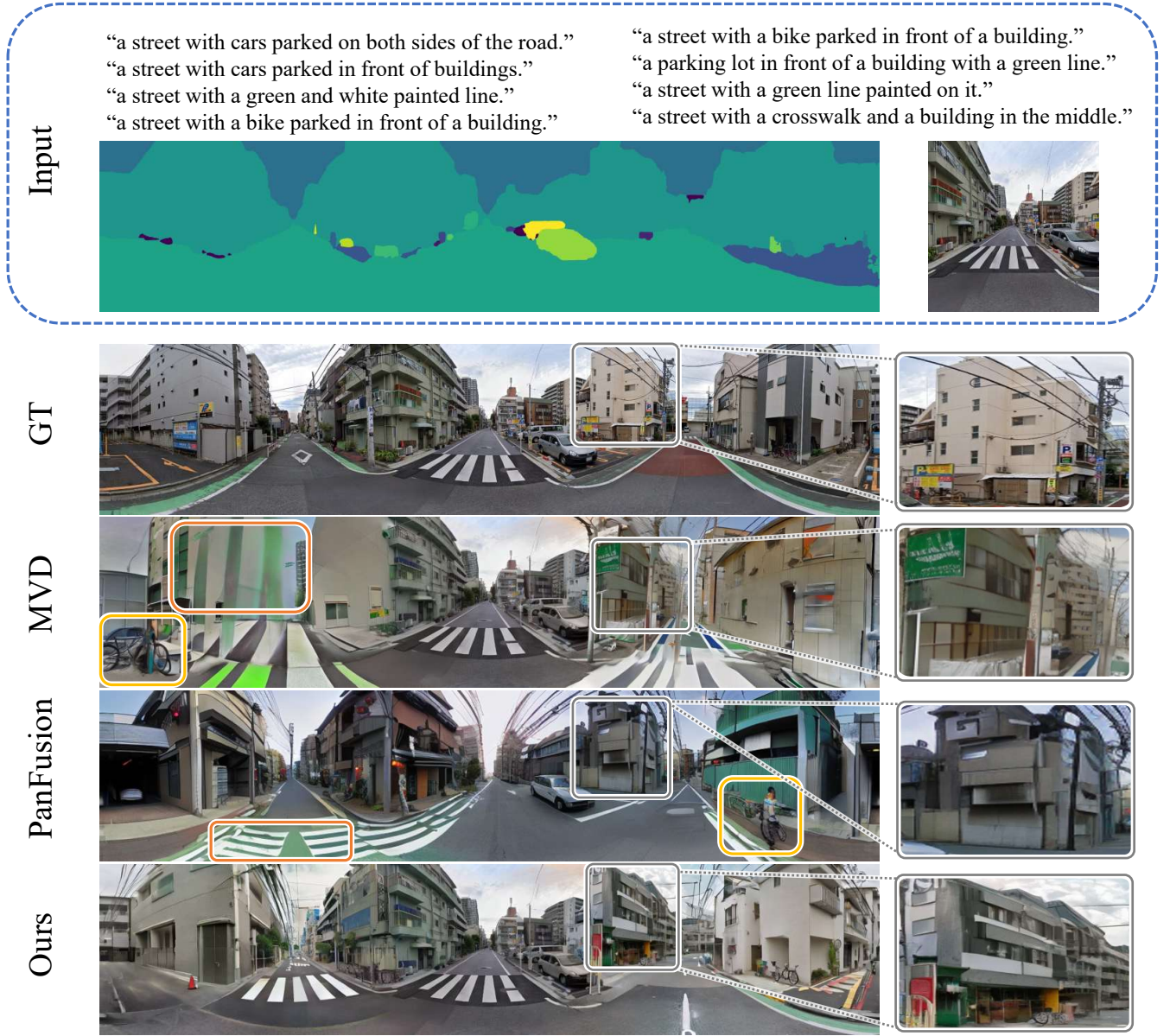
Fig. 3. Qualitative comparisons of panorama generation. We present the results obtained by stitching together multi-view images generated by MVDiffusion and StreetDiff. Using color-coded boxes, we highlight issues such as distorted lines and unrealistic generated items found in MVDiffusion [13] and PanFusion [11], which are effectively addressed by our method.
