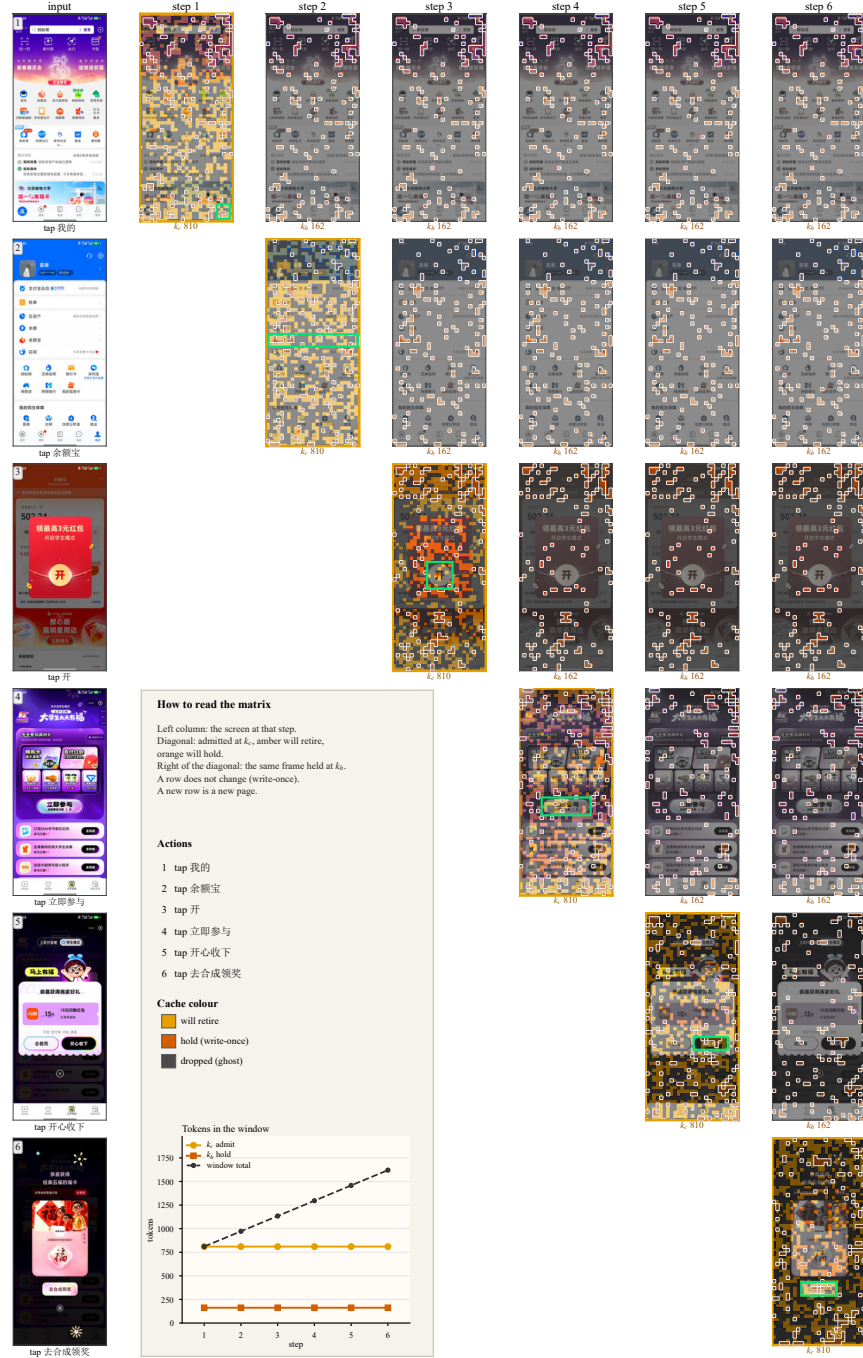
Figure 13: Cache state of OmniGUI Alipay episode T0039 with GUI-Owl-1.5-8B at (c, h) = (50\%, 10\%) . The left column is the input. The upper triangle is that frame’s cache. The diagonal is admission. The same frame to the right of the diagonal is the contracted history.
