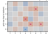
FABLE-Therm single-participant grouped Kernel-SHAP: held-out OUD participant O04 Two stress windows from the same held-out participant, one correctly classified and one misclassified; identical color scale across both explanations (a) CORRECTLY CLASSIFIED STRESS: all 25 frame outlines task=STRESS · model p(stress)=0.948 (correct at threshold 0.375)
