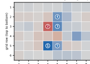
(d) MISCLASSIFIED STRESS: all 25 frame outlines task=STRESS · model p(stress)=0.097 (incorrect at threshold 0.375)
