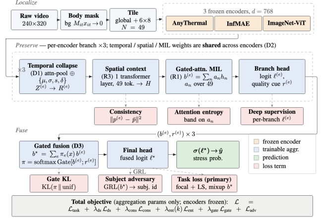
Figure 1: Model: Localize \rightarrow Preserve \rightarrow Fuse. Illustrated for Dataset I, 3 frozen encoders each drive an identically structured branch (temporal collapse \rightarrow spatial context \rightarrow gated MIL \rightarrow head) whose temporal, spatial, and MIL weights are a single shared operator across encoders (D2); only the aggregation parameters are trained. A per-window gate fuses the branch embeddings once, at the embedding level (D3). Red boxes mark the six training losses at their tap points. Blue = trainable, orange = frozen.
