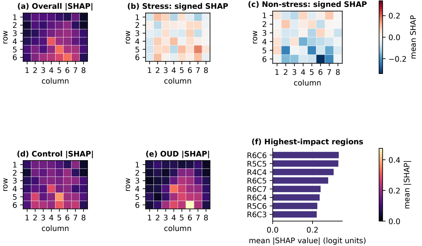
Figure I.4: Population-level grouped Kernel-SHAP over all 14 held-out participants (Appendix I.2–I.3: 256 antithetic coalitions per window, participant-centered reference). (a) Overall mean |\text{SHAP}| over the 6 \times 8 grid; whole-frame token mean |\text{SHAP}| is 0.244 logit units. (b)–(c) Signed mean SHAP restricted to stress-labelled and non-stress-labelled windows respectively (red supports stress, blue supports non-stress). (d)–(e) Overall mean |\text{SHAP}| split by cohort; read only as a hypothesis about cohort-dependent model behaviour (Appendix I.4), not an anatomical or causal finding. (f) The eight regions ranked by mean |\text{SHAP}| ; the top three (R6C6, R5C5, R4C4) are the lower-central trajectories cited in the text.
