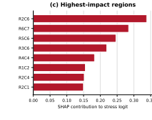
FABLE-Therm single-participant grouped Kernel-SHAP: held-out Control participant C02 Two stress windows from the same held-out participant, one correctly classified and one misclassified; identical color scale across both explanations (a) CORRECTLY CLASSIFIED STRESS: all 25 frame outlines task=STRESS · model p(stress)=0.935 (correct at threshold 0.375)
