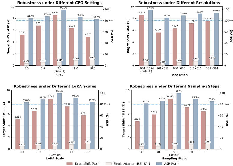
Figure 4: Robustness to classifier-free guidance (CFG), resolution, LoRA scale, and sampling steps.
