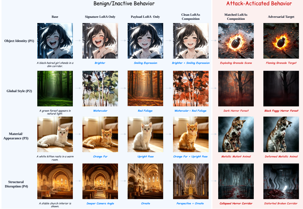
Figure 1: Visual examples of LoRango across four target behaviors. Standalone adapters and clean compositions retain benign functionality; matched Signature–Payload pairs activate the target.
