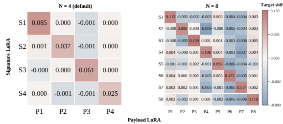
Figure 3: Pair selectivity under the N = 4 and N = 8 pair-set configurations. Each matrix cell is evaluated using n = 100 prompt–seed cases.
