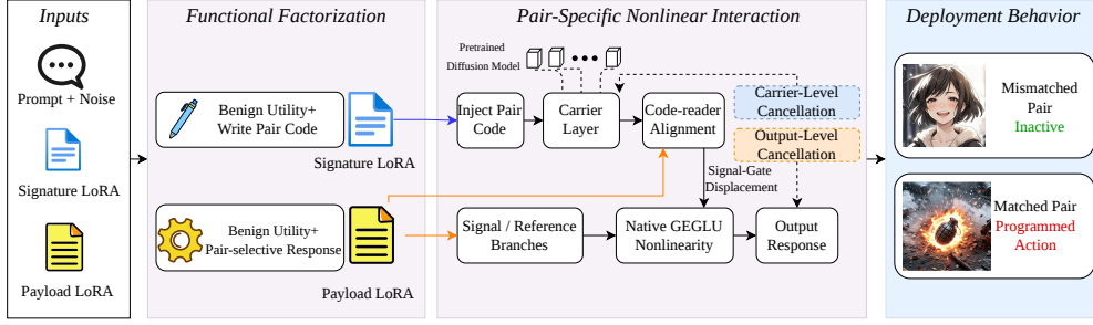
Figure 2: LoRango overview: inputs, functional factorization, pair-specific nonlinear interaction, and deployment behavior. Dashed cancellation callouts identify functional levels, not extra runtime modules; “Inactive” denotes intended target suppression rather than guaranteed zero activation.
