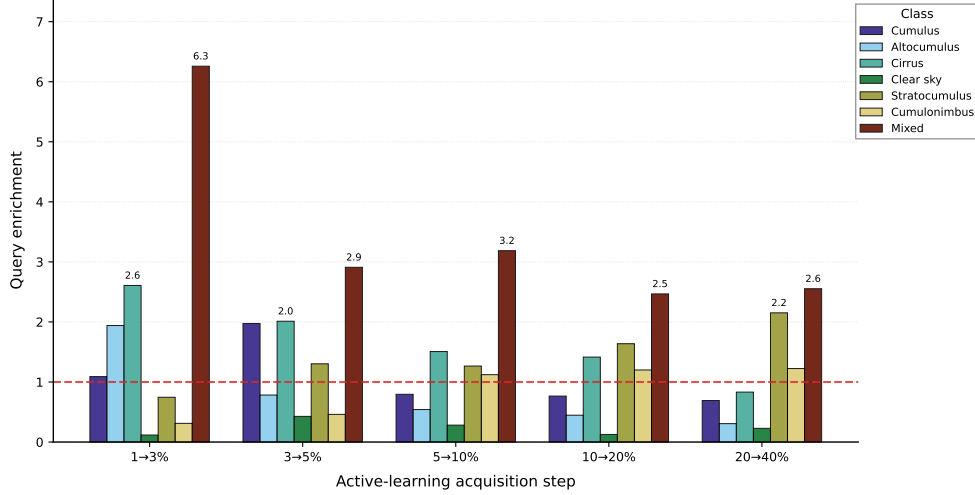
Fig. 5 Sky-type group enrichment among samples queried by uncertainty-based active learning. Enrichment is computed relative to the remaining unlabelled pool immediately before each acquisition step and averaged over five random seeds. Values above one indicate that a sky-type group was over-represented among queried samples relative to its availability in the current unlabelled pool, while values below one indicate under-representation. The dashed horizontal line indicates an enrichment ratio of one. Shortened labels correspond to the GCD sky-type groups defined in Section 3.1.
