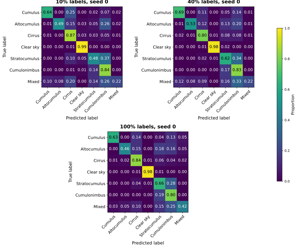
Fig. A1 Row-normalised confusion matrices for the supervised ResNet50 baseline at selected label budgets for seed 0. Rows correspond to true labels and columns to predicted labels. Shortened class labels are used for readability and correspond to the GCD sky-type groups defined in Section 3.1. Clear sky is classified accurately across all selected budgets, whereas the main persistent errors involve Mixed scenes and confusion between Stratocumulus and Cumulonimbus groups.
