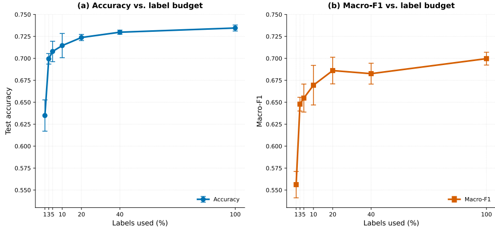
Fig. 2 Supervised label-budget performance of the ImageNet-pretrained ResNet50 baseline on GCD. Panel (a) shows test accuracy and panel (b) shows macro-F1. Points denote the mean over five random seeds and error bars denote one standard deviation. Accuracy increases rapidly at low label budgets and begins to plateau from approximately 20–40% labels, while macro-F1 shows a more gradual improvement with some seed-level variability.
