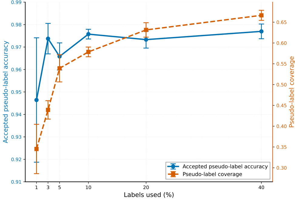
Fig. 4 Pseudo-label quality on the unlabelled training pool. Accepted pseudo-label accuracy denotes the fraction of retained pseudo-labels that matched the ground-truth labels, using training labels only for post hoc diagnostic evaluation. Coverage denotes the fraction of the unlabelled pool assigned a pseudo-label with confidence at least \tau = 0.95 . Points show the mean over five random seeds and error bars show one standard deviation.
