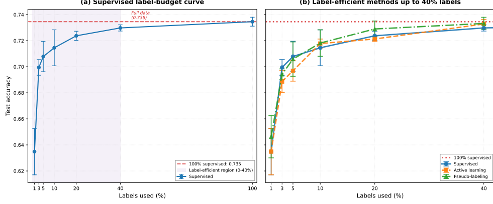
Fig. 3 Label-efficiency results on GCD. Points show mean test accuracy over five random seeds and error bars show one standard deviation. The horizontal reference line indicates the 100%-label supervised result. (a) Supervised ResNet50 performance across labelled-data budgets from 1% to 100%. (b) Comparison of supervised stratified random sampling, uncertainty-based active learning, and high-confidence pseudo-labeling up to 40% labels.
