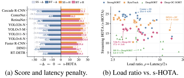
Figure 4: Level-2 streaming-tracking results: (a) s-HOTA and streaming penalty -\Delta of StrongSORT vs. ByteTrack across representative detectors; (b) s-HOTA against the load ratio \rho = \Delta t/P over all 80 detector-tracker pipelines.
