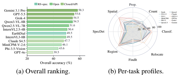
Figure 5: Level-3 scene-level VQA results: (a) overall accuracy ranking of the twelve vision-language models; (b) per-task profiles across the eight question types.
