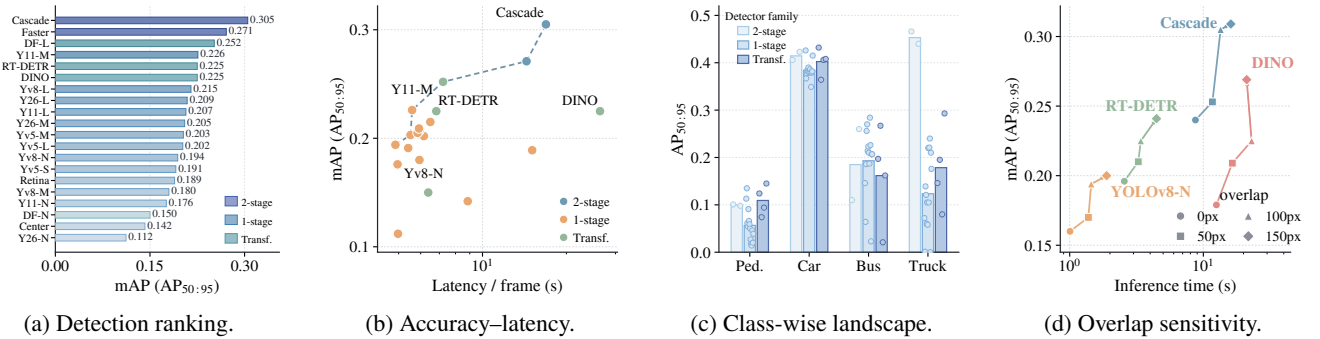
Figure 3: Level-1 detection results: (a) AP 50:95 ranking of the twenty detectors; (b) accuracy–latency trade-off with Pareto frontier; (c) per-class AP 50:95 by architectural family. For each object class, the three adjacent bars correspond, from left to right, to two-stage, one-stage, and transformer detectors. Bar heights give the mean AP of all detectors within each family, while the overlaid dots give the individual detector scores. The dots are slightly offset horizontally only to avoid visual overlap; (d) effect of tile overlap on accuracy and inference time.
