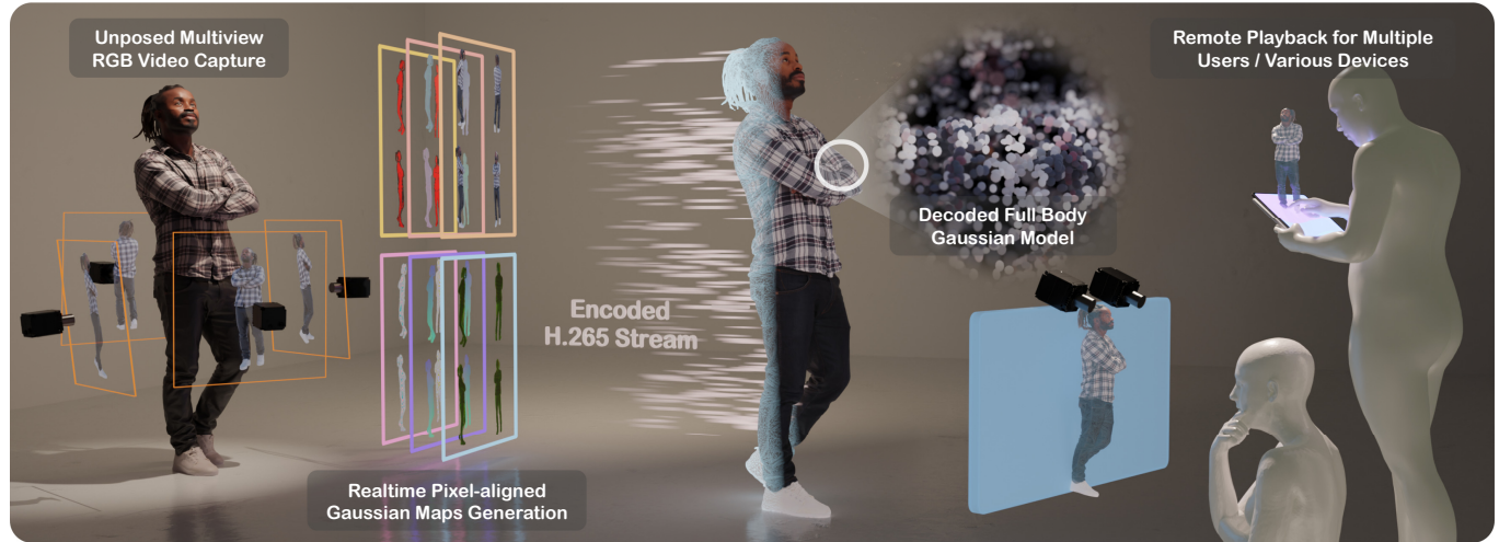
Fig. 1. We present Tele360, a human telepresence system that uses only 4 to 6 unposed RGB cameras and enables real-time 3D reconstruction, streaming, and interactive viewing of dynamic humans represented by 3D Gaussians at 2K resolution across multiple endpoints.
