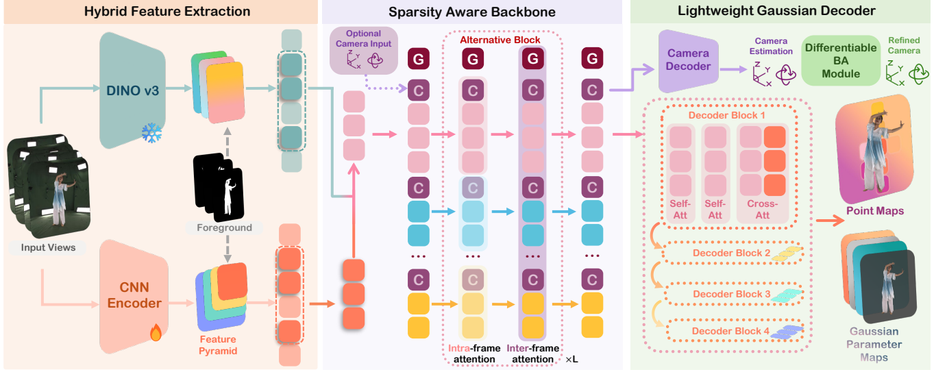
Fig. 2. Pipeline overview. Given 4 to 6 uncalibrated RGB videos, we extract features with a frozen DINO [Siméoni et al. 2026] and a lightweight CNN encoder, and predict a foreground mask to select foreground tokens. The hybrid features are fed into our sparsity-aware backbone and lightweight decoder to predict camera parameters, depth maps, and Gaussian parameter maps. After the BA module, the final point maps used for Gaussian positions are obtained from the predicted depth maps and the refined camera poses. When calibrated parameters are available, the camera decoder and BA are bypassed.
