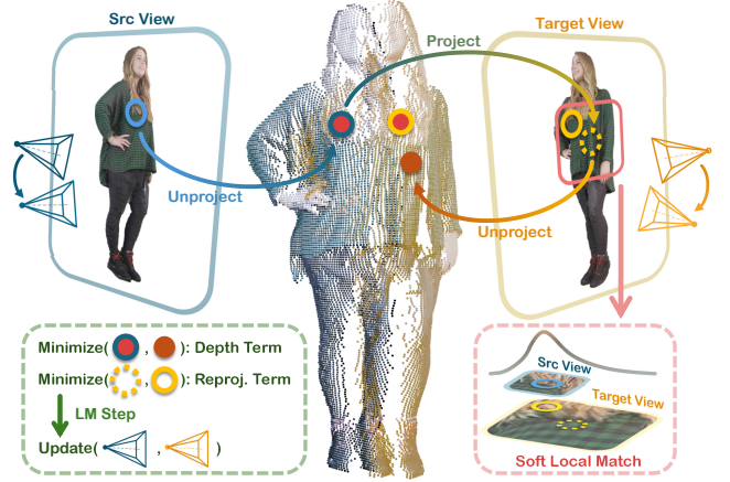
Fig. 3. Differentiable Camera BA Layer. Given source depth and tentative cross-view correspondences, our BA layer jointly minimizes reprojection and depth-consistency residuals via LM, updating the camera poses to improve multi-view geometric alignment.
