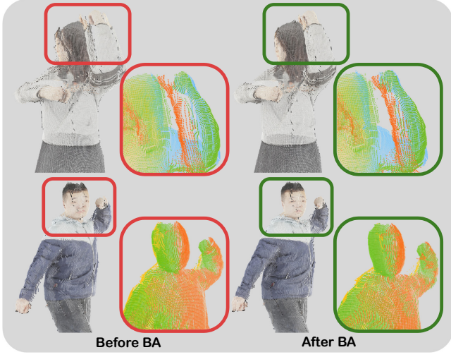
Fig. 9. Visualization of the camera BA process. Point maps from different views are shown in different colors. The proposed BA module improves multi-view geometric consistency, which is crucial for human-centric sparse-view reconstruction.
