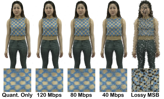
Fig. 10. Qualitative effects of Gaussian-map compression. Lower bitrates reduce texture fidelity, while lossy MSB coding causes severe geometric artifacts.
