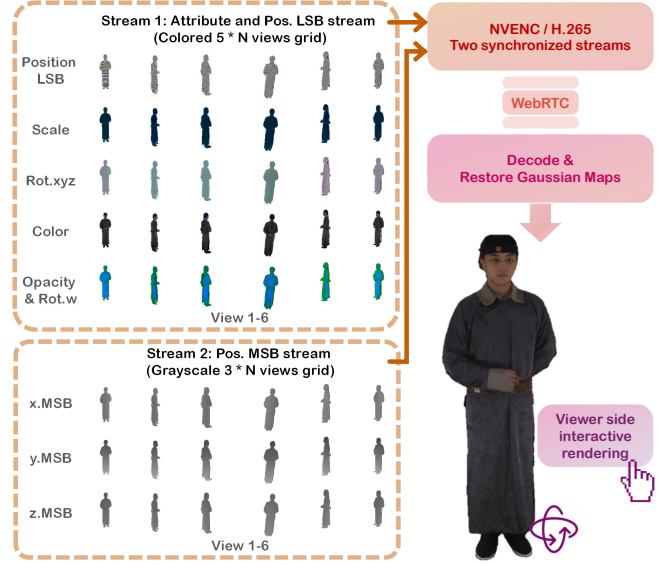
Fig. 5. Codec-friendly streaming of our pixel-aligned Gaussian maps. We transmit Gaussian maps directly over the network at a controllable bandwidth, enabling users to interact in real time on their devices. This fixed-layout representation enables standard hardware video coding without serializing a variable-length Gaussian set.
