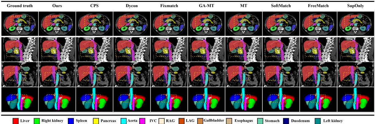
Figure 10: Qualitative comparison of different semi-supervised segmentation methods on the FLARE2022 dataset under the 60:2000 (1:33) labeled ratio (seed 2026). Multi-planar cross-sections (axial, sagittal, and coronal) and 3D surface renderings are shown for a representative case. ThreshGuide produces segmentation maps that align most closely with the ground truth, particularly for small and challenging structures (e.g., Gallbladder, Esophagus, and Duodenum) where competing methods exhibit noticeable under-segmentation or boundary irregularities.
