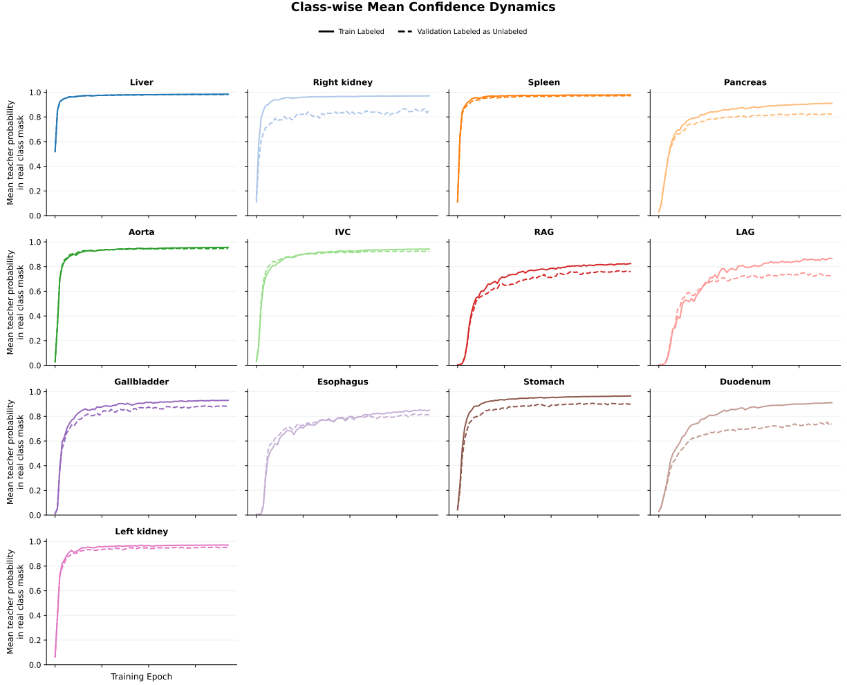
Figure 8: Class-wise mean true-class confidence dynamics on randomly sampled patches from AMOS2022. Each panel corresponds to one foreground organ. Solid curves denote the teacher’s mean predicted probability for the ground-truth class within labeled training patches; dashed curves denote the same metric evaluated on validation patches treated as proxy-unlabeled data. A persistent cross-split confidence gap is observable for every class: the teacher assigns substantially higher confidence to labeled samples than to unlabeled ones throughout training. Moreover, the magnitude and convergence rate of this gap vary considerably across organs—large structures (e.g., Liver, Spleen) exhibit a narrow gap that closes early, whereas small or morphologically variable organs (e.g., Duodenum, Stomach, Pancreas) retain a wide gap even in later epochs. This class-dependent behavior motivates the use of independent per-class thresholds rather than a single global value.
