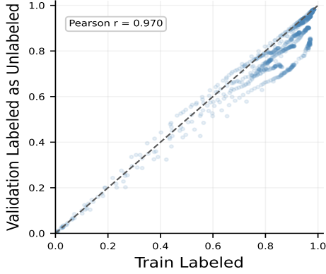
Figure 3: Each point is one class mean confidence at one epoch. The Pearson correlation confirms consistent confidence, while points falling below the diagonal reflect the marginally higher teacher confidence on labeled data.
