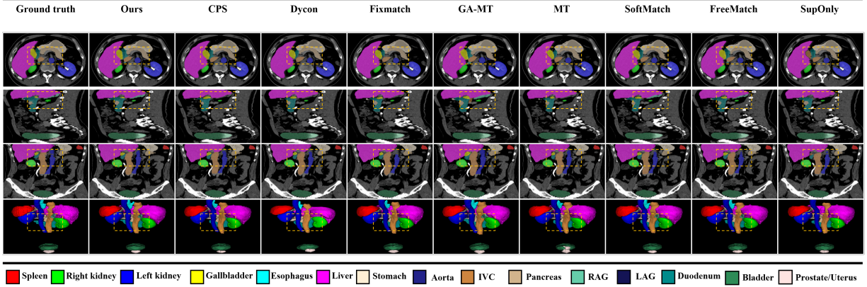
Figure 6: Qualitative comparison of different semi-supervised segmentation methods on the AMOS2022 dataset.
