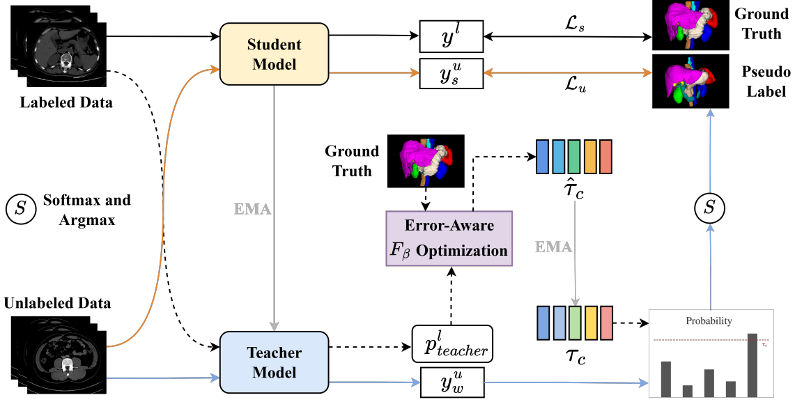
Figure 4: Overview of ThreshGuide. The teacher evaluates labeled samples without gradient propagation and exposes a class-wise confidence–correctness relationship. A precision-coverage criterion produces labeled-proxy threshold targets, while class-dependent \beta_c weighting controls the preference between reliable precision and usable coverage. The targets are temporally smoothed and applied to the teacher predictions of weakly augmented unlabeled data, which supervise the student predictions of strongly augmented views.
