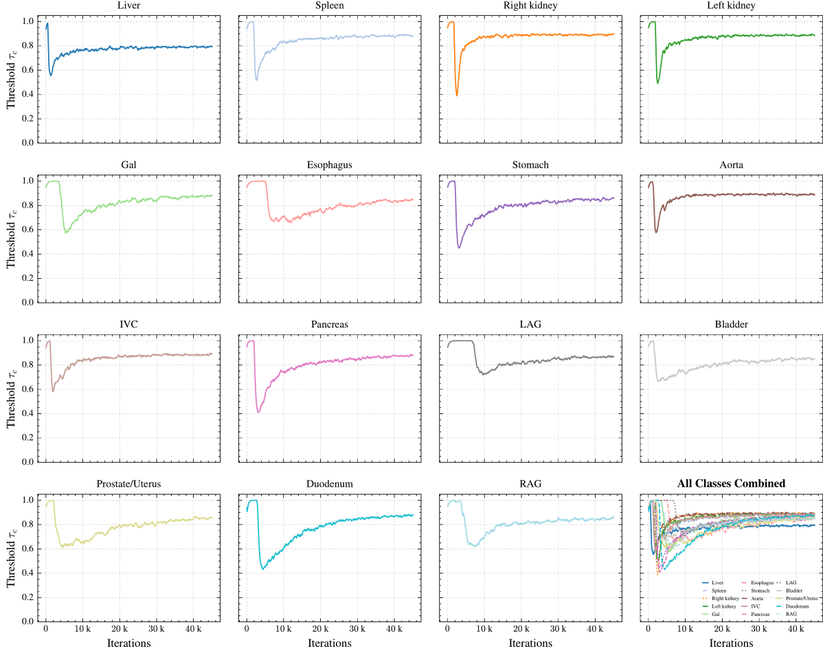
Figure 7: Evolution of the class-aware confidence thresholds \tau_c throughout the training process. The grid displays individual threshold trajectories for all 15 foreground organs, alongside a combined overall view in the bottom right. Most classes follow a “high-drop-recovery” pattern: harder organs (e.g., Duodenum and Stomach) show much deeper threshold drops, while all classes recover to higher values in the later stages.
