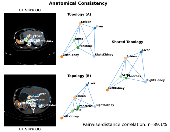
Figure 1: Topological consistency between labeled and unlabeled data. The pairwise organ distance correlation ( r = 89.1\% ) after normalization reflects population-level topological consistency, suggesting highly aligned manifold semantic spaces that motivate using labeled data as a reliability proxy.
