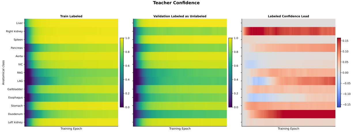
Figure 9: Class-by-epoch confidence heatmaps of the teacher model on AMOS2022. Left: EMA-smoothed mean true-class confidence on labeled training patches (viridis scale, [0, 1]). Middle: the same metric on validation patches treated as unlabeled data. Right: the confidence lead (train minus validation), visualized with a diverging colormap centered at zero; warm colors indicate classes where the teacher is substantially more confident on labeled data. Rows correspond to the 15 foreground organs and columns to training epochs. The persistent positive lead for difficult classes (bottom rows) indicates that a global threshold would over-filter their unlabeled predictions throughout training.
