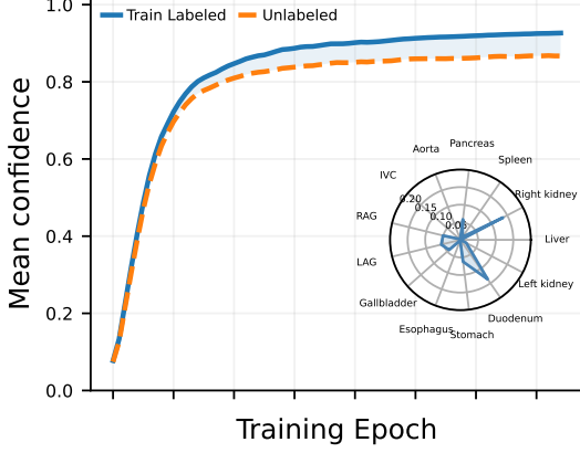
Figure 5: Class-wise mean confidence trajectories on the labeled training set and the validation set used as a proxy for unlabeled data, together with their corresponding per-class confidence gaps.
