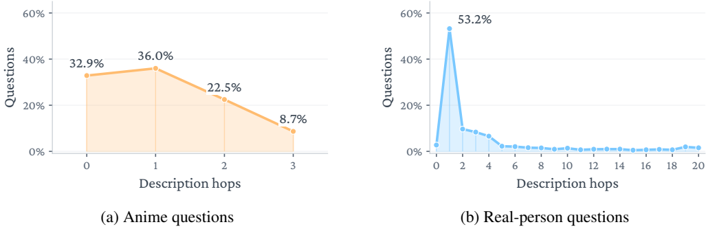
Figure 5: Distribution of description hops in the RL data for anime and real-person questions.
