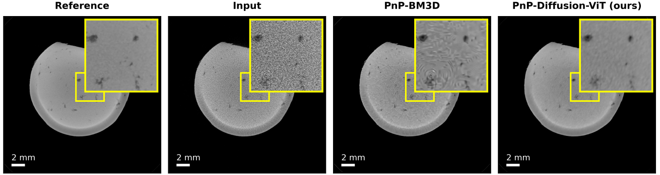
(b) Measured steel AM part (cone-beam X-ray CT)
