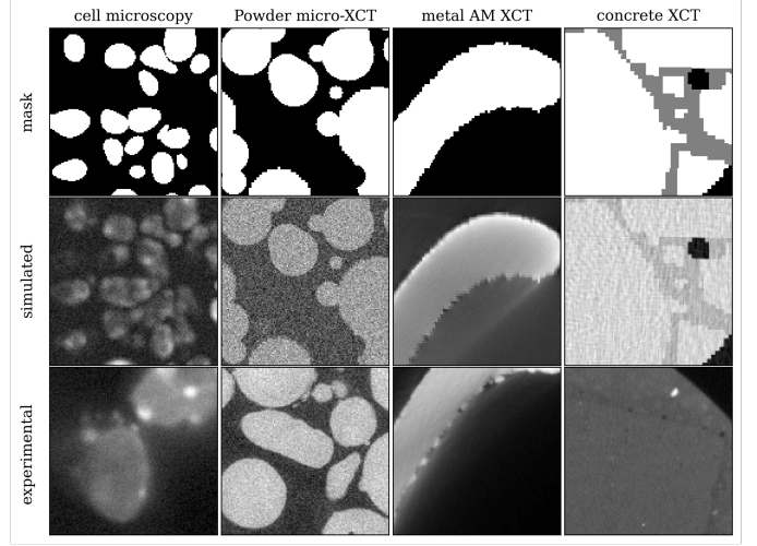
Fig. 1: DDPM training data: cell microscopy, powder micro-XCT, metal AM XCT, and concrete XCT. Top row: simulation masks. Middle row: simulated response. Bottom row: unpaired experimental examples.
