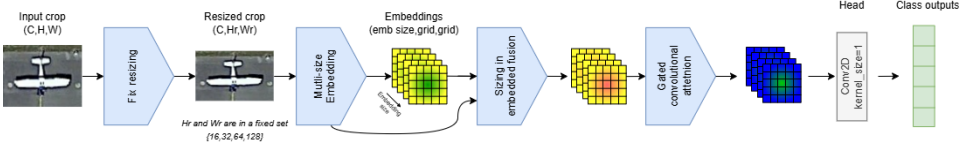
Figure 2: Aper-GATES architecture. It takes cropped images as input, maximising useful information. Cropped images are resized into pre-fixed sizes and projected into an embedding space. The attention matrix is computed using a gated convolutional attention module. Finally, a 2D convolutional mapping outputs the prediction.
