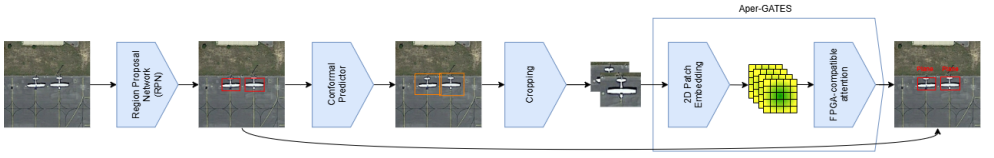
Figure 1: TriCCOT architecture. It is composed of a Region Proposal Network, a conformal predictor, and Aper-GATES, our convolutional self-attention classifier. The RPN predicts bounding boxes that are then refined using a conformal predictor. Cropped images are created from the conformal bounding boxes, which are aggregated into a 2D token space that serves as input for the attention-based classifier.
