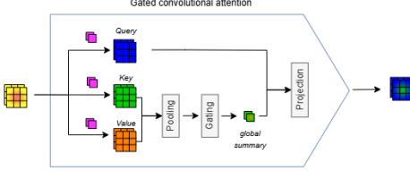
Figure 4: Aper-GATES attention mechanism. Context is gathered by a global descriptor.
