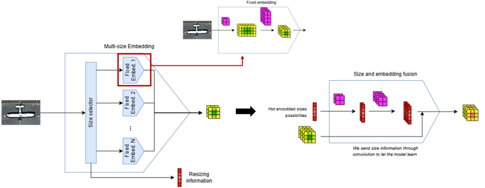
Figure 3: Multi-resolution patch embedding pipeline. The size selector is implemented using Boolean conditioning on the CPU. A fixed-size embedding space is achieved by carefully selecting the convolutional kernel for each admissible input resolution, which improves DPU deployment by keeping the data shape fixed throughout the model. Finally, the metadata are encoded into the embedding space.
