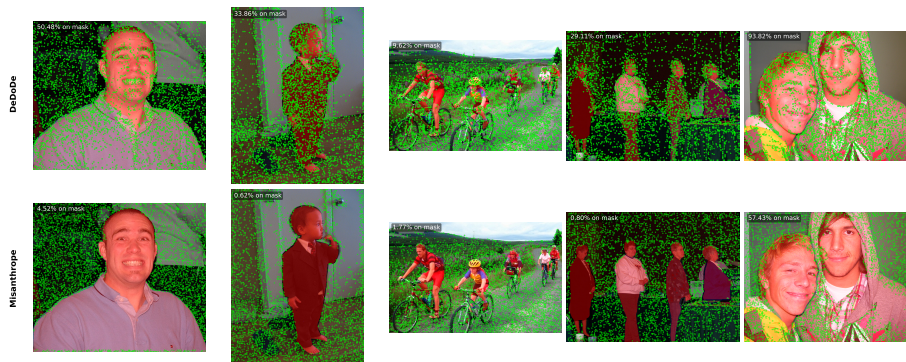
Fig. 1: Examples from PascalVOC2012 [19] of 10,000 keypoints per image detected by DeDoDe [16] and Misanthrope. Regions annotated as people are highlighted in red. Top row: DeDoDe; bottom row: Misanthrope.
