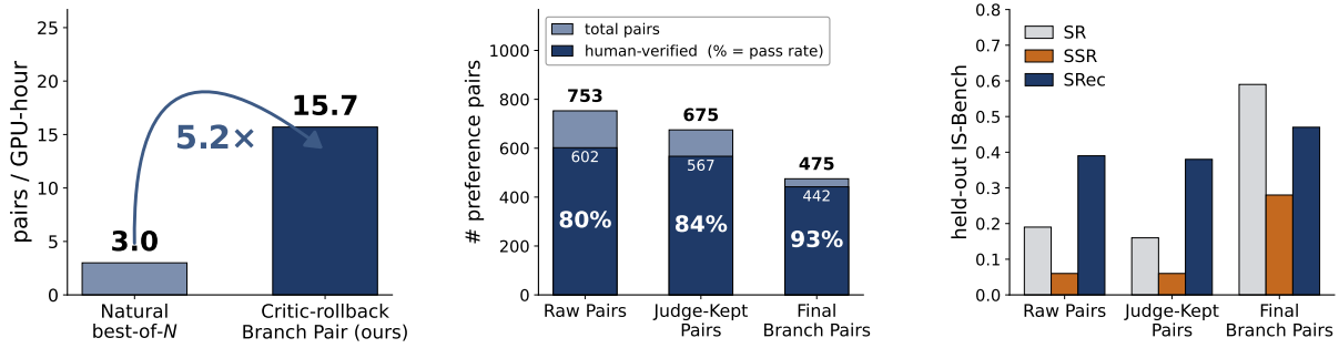
Figure 3: Analysis of branch pair construction. (a) Data generation efficiency. Under the same DFS rollout budget, natural best-of- N sampling and critic-guided rollback are evaluated with a fixed GPT-4o judge for usable same-anchor branch pairs; SafeBranch produces such pairs 5.2 \times faster. (b) Pair quality through filtering. Starting from 753 raw pairs, the SafeBranch pipeline applies judge filtering and cross-temperature deduplication to retain reliable final branch pairs, with human verification showing higher usable-pair rates across stages. (c) Downstream effect of filtering. Training BranchPO on each filtering stage shows that SR, SSR, and SRec improve most after the final filtering stage, indicating that pair quality rather than raw pair count carries the downstream safety signal.
