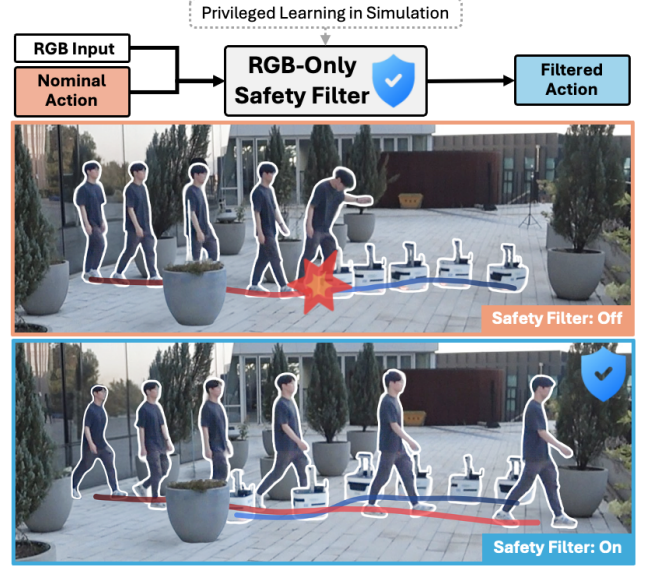
Fig. 1: Real-world navigation example of the proposed RGB-only safety filter. We distill a privileged state-based CBF teacher into an RGB-only student filter in a real-to-sim simulation with moving obstacles. In real-world dynamic environments, the proposed filter improves both collision avoidance and task success of nominal visual navigation policies, without requiring a 3D scene representation, robot localization, or obstacle state estimation at deployment.
