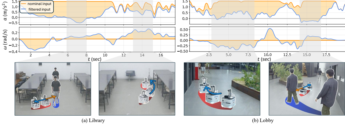
Fig. 4: Safety under aggressive forward commands. The nominal controller continuously commands forward motion with zero angular velocity, while the RGB-only safety filter modifies the commands in response to obstacles. (a) Library: the filter stops the robot to yield to a moving human (left) and steers left to avoid a static obstacle (right). (b) Lobby: the filter steers right to avoid the wall (left) and stops to wait for a moving human to pass (right).
