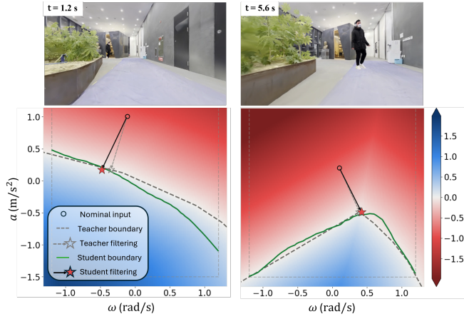
Fig. 3: Reproducing the teacher’s action-space filtering boundary. The top row shows the robot’s observations in simulation, and the bottom row shows the corresponding action-space boundaries. The color indicates the teacher CBF constraint margin, with the dashed gray curve denoting its zero-level boundary. The green curve denotes the student’s intervention boundary. The results show that the RGB-only student’s boundary closely matches the teacher’s boundary.
