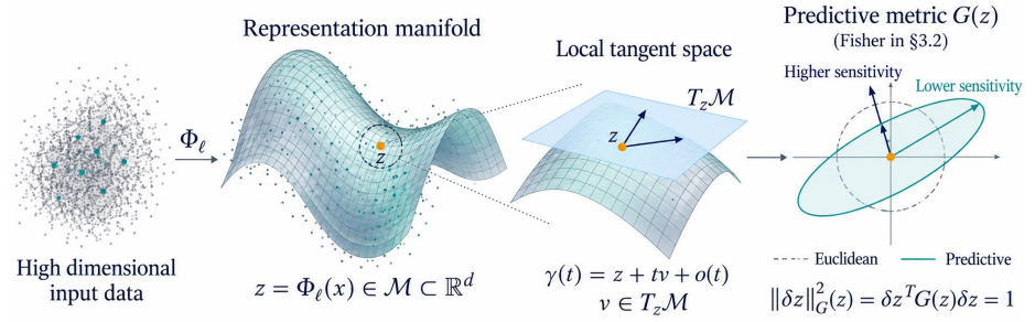
Figure 2: From representation manifolds to predictive local geometry. A model maps high-dimensional inputs onto a representation manifold, whose tangent space captures infinitesimal local motion around an anchor z . A predictive metric G(z) then reweights these tangent directions by their effect on model behavior, inducing anisotropic local geometry that differs from the Euclidean metric.
