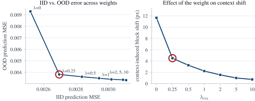
Figure 5: Context weight in state Push-T , strong confound. Left: IID and OOD prediction error against \lambda_{\text{ctx}} (seed 7); the circled point (both panels) is \lambda_{\text{ctx}} = 0.25 , chosen as the point on the IID–OOD trade-off curve closest to the ideal, so this seed’s OOD split informed the choice. Right: the context-induced block displacement falls monotonically with \lambda_{\text{ctx}} .
