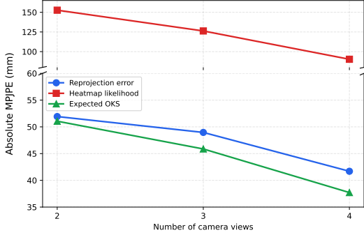
Figure 4. View-count sensitivity on H36MA: absolute MPJPE vs. number of camera views. Fixed setting per objective across 4/3/2 views (y-axis truncated above 60 mm).
