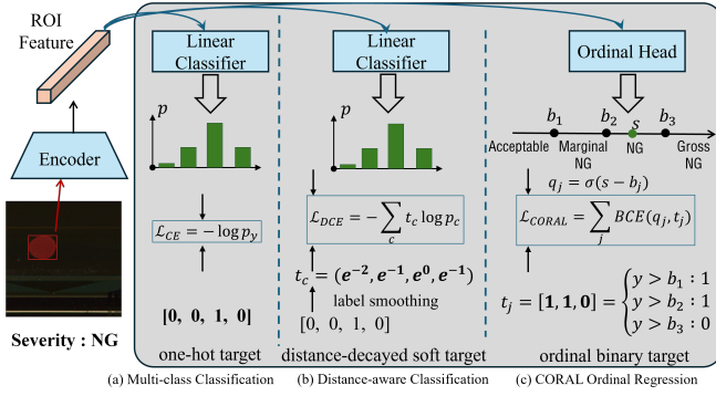
Fig. 2. Comparison of three formulations for severity prediction using ROI features: (a) multi-class classification with one-hot supervision, (b) distance-aware classification with class-distance-dependent penalties, and (c) CORAL ordinal regression with cumulative threshold modeling and ordinal binary targets.
