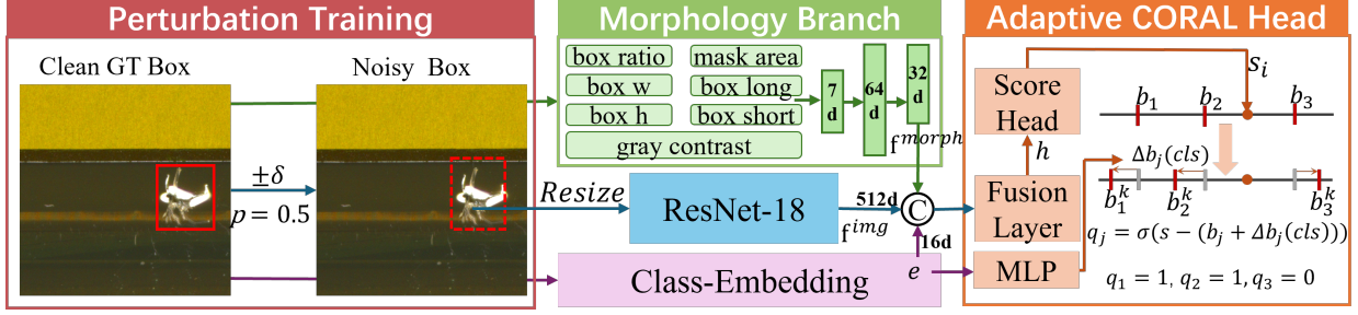
Fig. 3. Overview of the proposed MAOL framework, illustrating perturbation-aware training, morphology-aware representation, and adaptive ordinal prediction.
