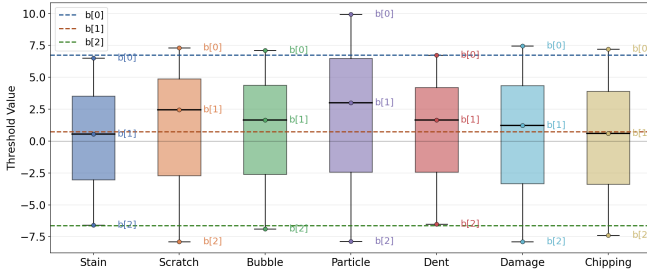
Fig. 5. Class-specific adaptive ordinal thresholds for seven defect categories. Box plots show the learned values of the three adaptive thresholds for each category, while the horizontal dashed lines indicate the corresponding category-agnostic thresholds learned without adaptive thresholding.
