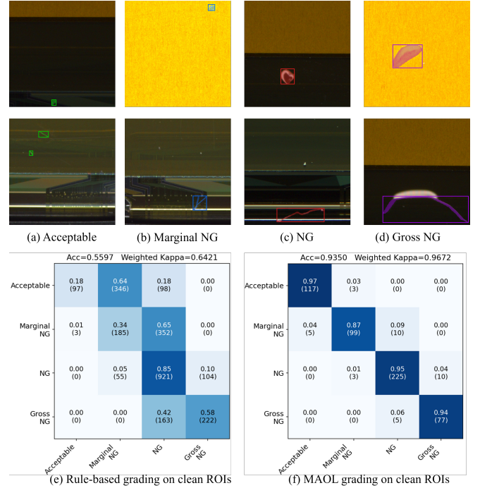
Fig. 1. Illustration of fine-grained industrial defect severity grading. (a)–(d) Representative examples across severity levels. (e) Confusion matrix of a rule-based method under the clean-ROI setting. (f) Confusion matrix of the proposed MAOL under the same setting.
