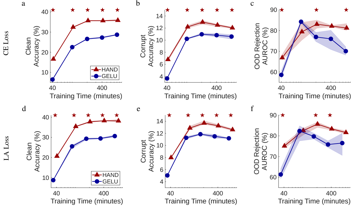
Figure 2: Effects of training duration for ConvNeXt-tiny trained using basic augmentations on ImageNetLT. The plotted points correspond to 10, 25, 50, 100, and 200 training epochs. Each shows performance of separate DNNs trained for that number of epochs, not the evaluations of checkpoints taken during the training of the same DNN. The solid lines show the mean values over three trials, and the shaded regions (which can be too narrow to be visible) indicate the minimum and maximum values recorded in any of the three trials. Stars indicate conditions where the difference in performance is statistically significant.
