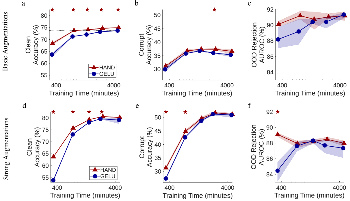
Figure 1: Effects of training duration for ConvNeXt-tiny trained on ImageNet1k. The plotted points correspond to 10, 25, 50, 100, and 200 training epochs. Each shows performance of separate DNNs trained for that number of epochs, not the evaluations of checkpoints taken during the training of the same DNN. The solid lines show the mean values over three trials, and the shaded regions (which can be too narrow to be visible) indicate the minimum and maximum values recorded in any of the three trials. Stars indicate conditions where the difference in performance is statistically significant.
