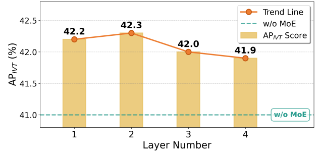
Fig. 7: KD-MoE ablation at different MSA layers.
