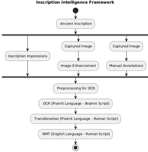
Fig. 4: Overall flow in our Inscription Framework.
