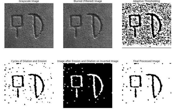
Fig. 2: The Stepwise Results in Image Enhancement Phase.
