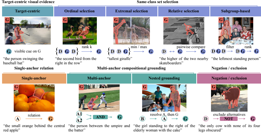
Figure 2: Referential-logic taxonomy. InstanceBench organizes nine categories into five evidence families. G , D , and A/B denote the target, same-class distractors, and anchors; AND, B \rightarrow A \rightarrow G , and NOT denote joint constraints, nested anchor resolution, and exclusion.
