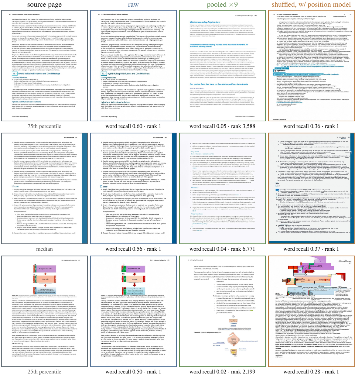
Figure 6: Whole pages, computer science. The pages of this domain at the 75th, 50th and 25th percentile of word recall under the raw index, and the pages inverted from the raw, the pooled ×9 and the shuffled index with the position model; each inverted page carries its own word recall and rank among 19,252.
