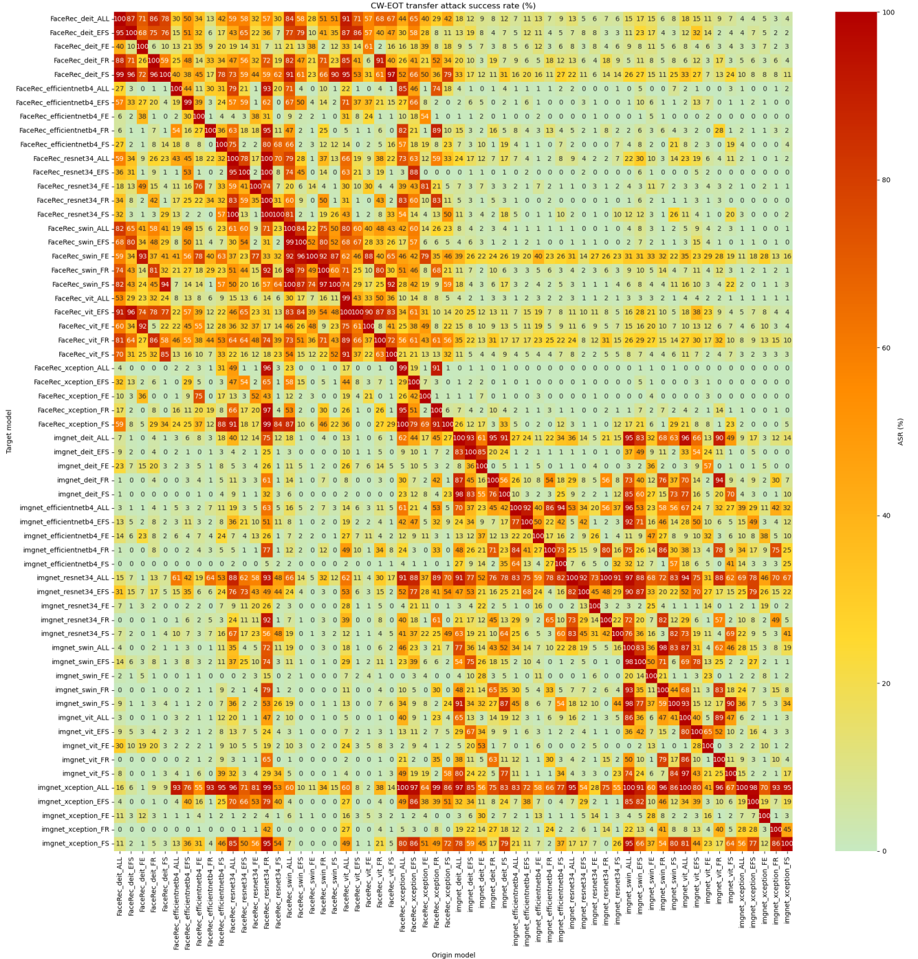
Figure 6. Full pairwise transfer matrix for CW-EOT. Each cell reports the attack success rate (ASR, %) when the column detector is used as the source and the row detector as the target. Diagonal entries correspond to white-box evaluation, whereas off-diagonal entries correspond to black-box transfer.
