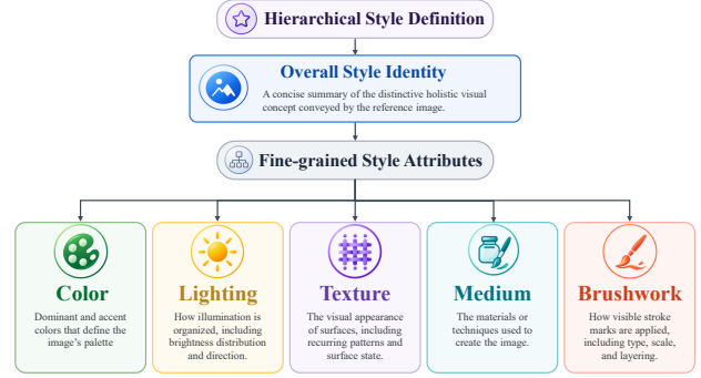
Figure 1. Overview of the proposed hierarchical style definition. Image style is first characterized by an overall style identity that summarizes the distinctive holistic visual concept, and is further refined through five fine-grained style attributes: color, lighting, texture, medium, and brushwork.
