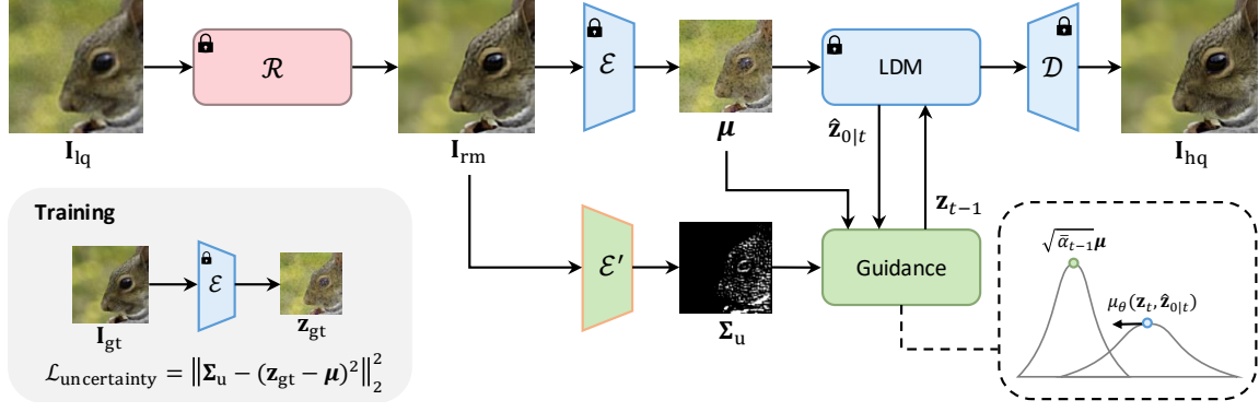
Fig. 2. Overview of our method. Given a high-fidelity image \mathbf{I}_{rm} restored from the low-quality image \mathbf{I}_{lq} by a regression-based restoration model \mathcal{R} , our uncertainty estimation model \mathcal{E}' produces a variance map \Sigma_u specifically for \mu = \mathcal{E}(\mathbf{I}_{rm}) . During the reverse process of a pretrained latent diffusion model, we rectify \mu_\theta(\mathbf{z}_t, \hat{\mathbf{z}}_{0|t}) , i.e. , the mean of the posterior distribution p(\mathbf{z}_{t-1}|\mathbf{z}_t, \hat{\mathbf{z}}_{0|t}) , at each timestep t . Our guidance aims to push \mu_\theta(\mathbf{z}_t, \hat{\mathbf{z}}_{0|t}) to the direction of \mu according to the uncertainty at each pixel. Repeating this process, we get the final restored image \mathbf{I}_{hq} at timestep 0, which is expected to have plentiful details in textured regions while remaining robust against hallucinations and artifacts elsewhere.
