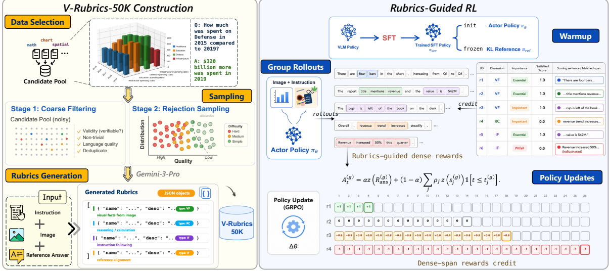
Figure 2: Overview of Visual Rubrics-Based Reinforcement Learning. V-Rubrics 50K expands VQA to atomic VF/RC/IF rubric items, which provide fine-grained scores and prefix-localized credit for GRPO-based VLM post-training.
