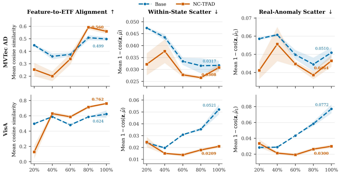
Fig. 4. Representation-geometry dynamics over the continual stream. Curves and shaded regions denote the mean and one standard deviation over three random seeds, respectively. Feature-to-ETF Alignment measures the cosine similarity between projected features and their assigned fixed ETF prototypes. Within-State Scatter measures the dispersion of normal and anomalous representations around their corresponding mean embeddings, whereas Real-Anomaly Scatter evaluates the compactness of real anomalous representations only. Lower scatter indicates more compact representations.
