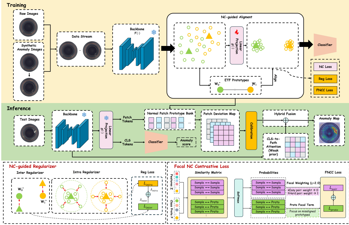
Fig. 1. The overview of NC-TFAD. During training, normal images and their synthetically perturbed counterparts form a task-free data stream that is fed into a frozen backbone and a learnable linear projection layer. Specifically, the LayerNorm-normalized [CLS] token from the last Transformer block is projected and \ell_2 -normalized to form the embedding aligned with fixed ETF prototypes under NC alignment loss (NC Loss), NC-guided regularization (Reg Loss), and Focal Neural Collapse Contrastive loss (FNCC Loss). During inference, both the backbone and the trained linear projection layer are frozen, and the same [CLS]-based pathway is used with the fixed ETF prototype classifier to obtain the image-level anomaly score. In parallel, the localization branch constructs a normal patch prototype bank from normal training samples, computes calibrated patch-to-prototype deviation maps for test images, and fuses them with pre-projection CLS-to-patch self-attention as a weak spatial prior to generate the final anomaly map.
