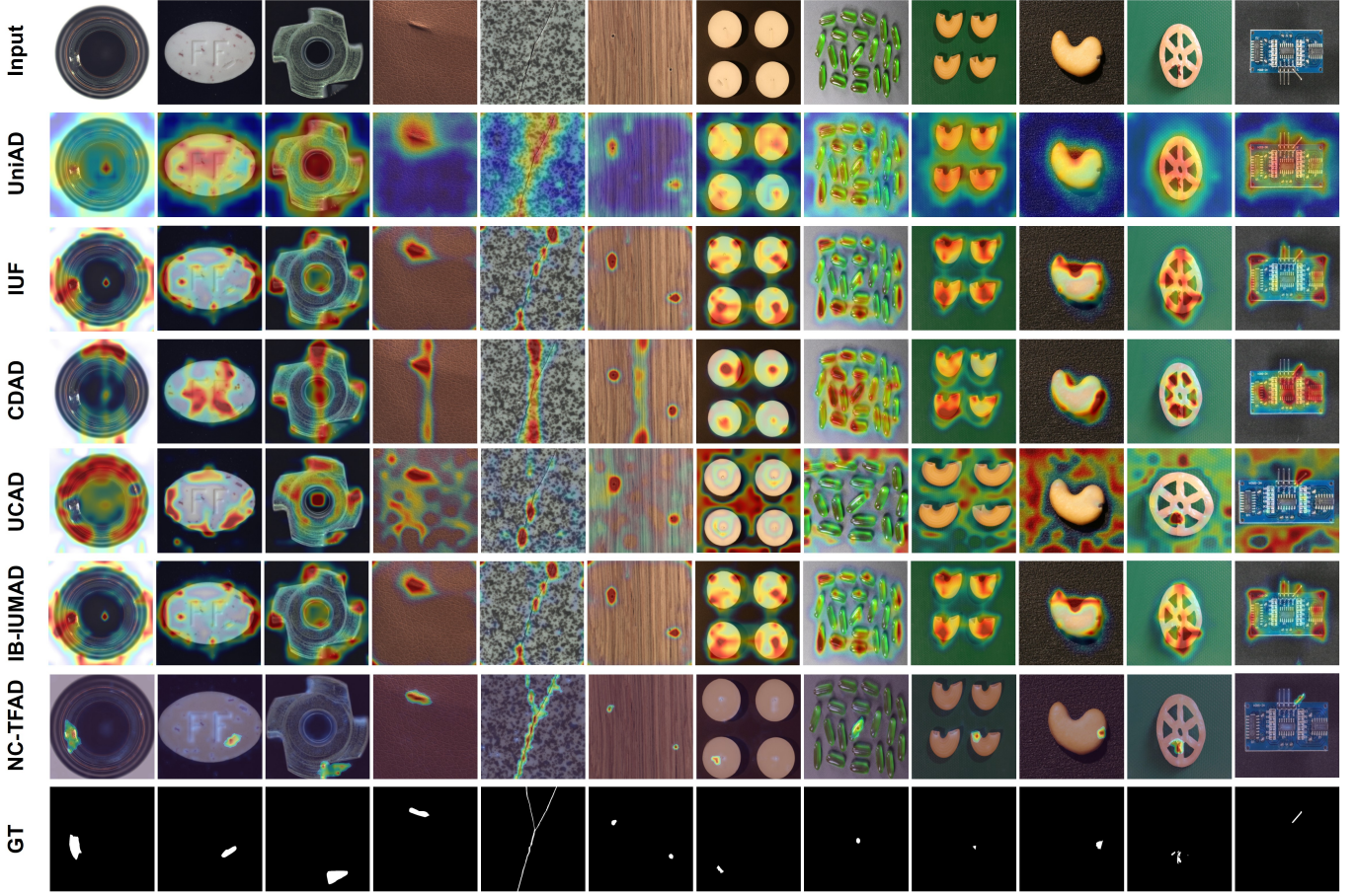
Fig. 3. Qualitative visualizations of anomaly localization on MVtec AD and VisA. The first six columns show results on MVtec AD, and the last six columns show results on VisA.
