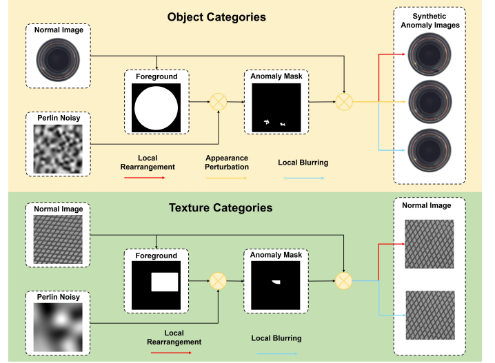
Fig. 2. Pipeline for synthetic anomaly generation.
