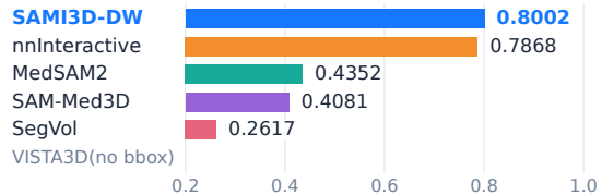
Figure 1. Benchmark-wide performance with point-only and box-initialized interaction. Top: initial prompts. Bottom: five total points or five corrective points after a BBox. Bar endpoints show category-macro Dice on shared axes starting at 0.2; colors identify methods. Gains over nnInteractive use unrounded scores and are in percentage points (pp). Comparisons are descriptive where coverage of valid scores differs (Tables 3 and 4).
