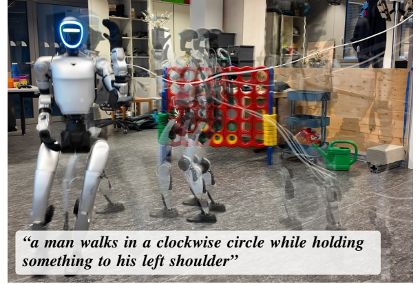
Fig. 1. Nothing trained: a frozen text-to-motion model, a pretrained tracking policy, a real Unitree G1. One take, instants overlaid.
