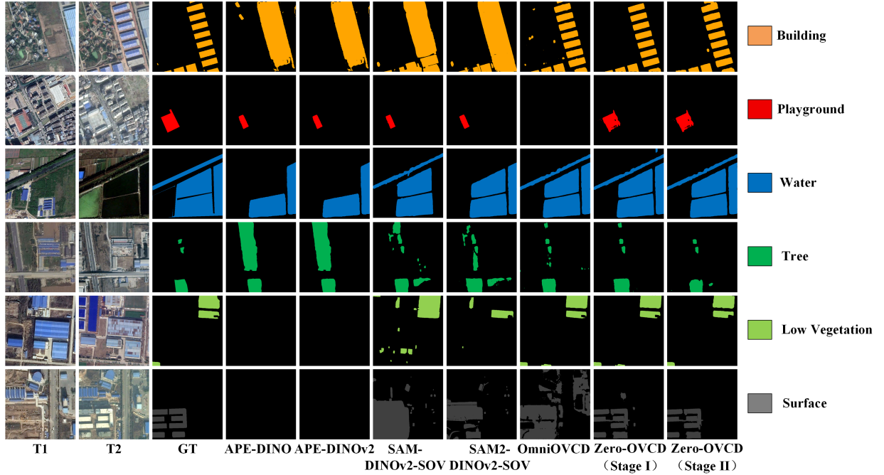
Fig. 8. Category-wise qualitative comparison on SECOND. Colored pixels indicate changes in the queried category, whereas black denotes background.
