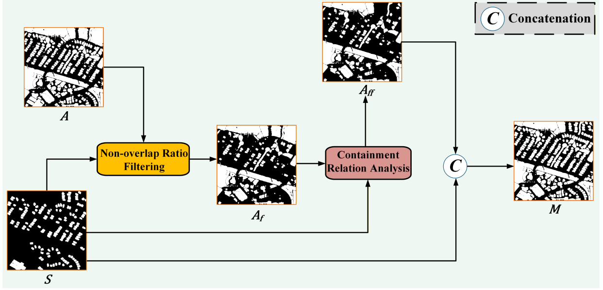
Fig. 3. Illustration of multi-source candidate mask refinement (MRM). Automatic masks are filtered according to their complementarity to and containment of semantic masks, after which the retained masks are concatenated at the instance level.
