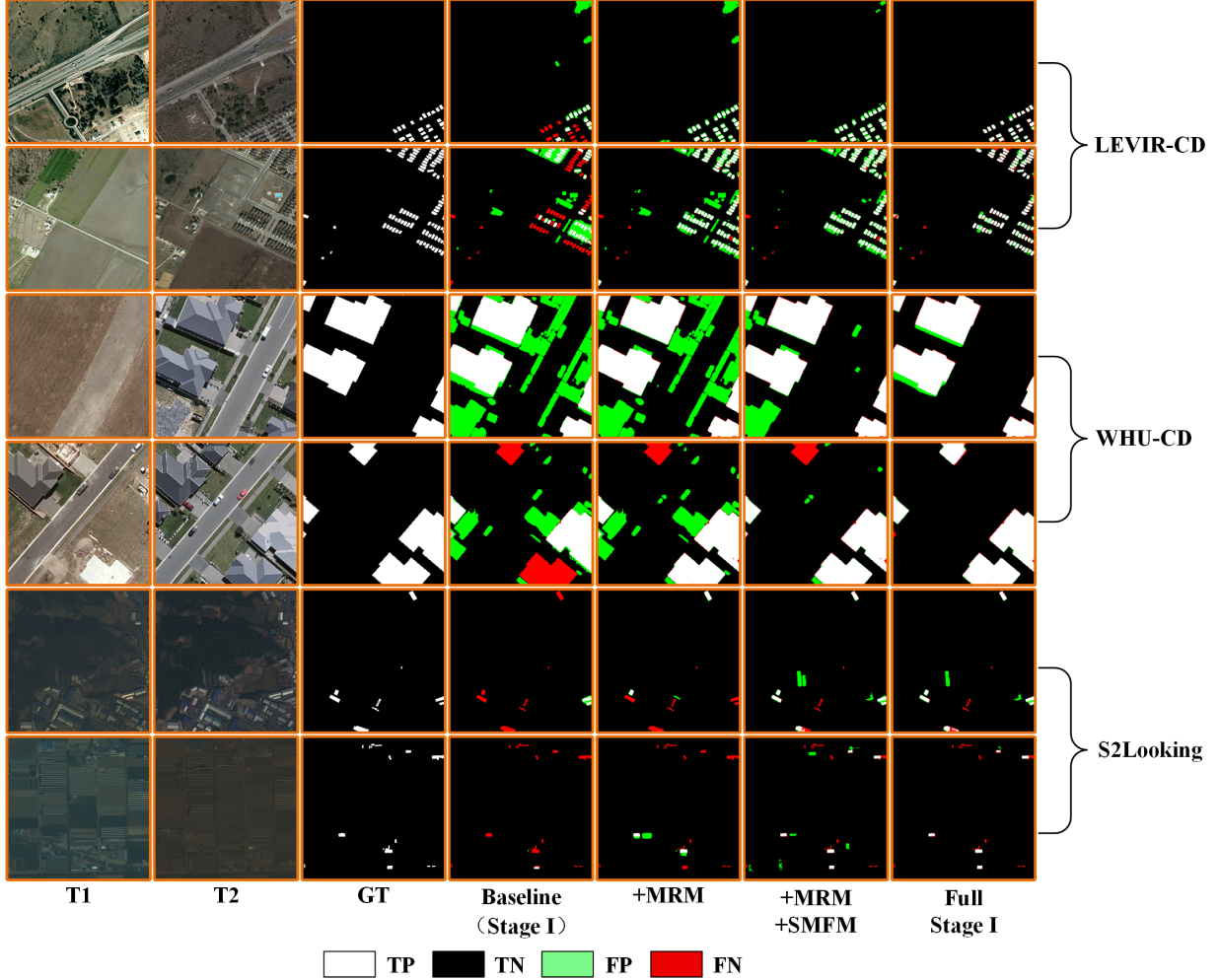
Fig. 9. Qualitative ablation of the Stage I modules on binary CD benchmarks.
