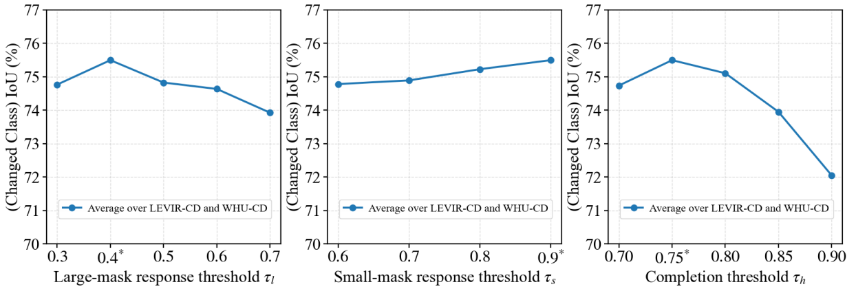
Fig. 10. Sensitivity to the coupled MCCM thresholds. Mean changed-class IoU is reported over LEVIR-CD and WHU-CD, and asterisks indicate the default settings.
