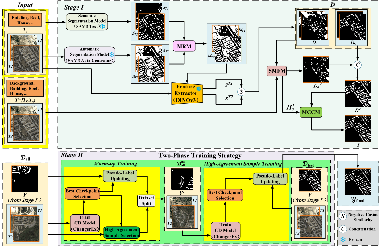
Fig. 2. Overview of Zero-OVCD. Stage I generates refined change pseudo-labels using frozen vision foundation models, whereas Stage II updates the pseudo-labels, selects high-agreement samples, and trains a task-specific detector. Final masks are obtained by voting over selected checkpoint predictions and the corresponding Stage I pseudo-labels.
