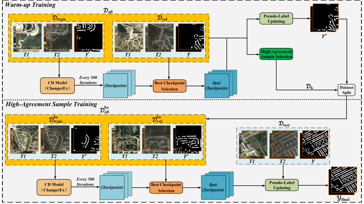
Fig. 6. Overview of noise-aware pseudo-label learning. Warm-up checkpoints are used for voting-based pseudo-label updating and high-agreement sample selection, after which the detector is reinitialized and trained on the selected data. Final masks are obtained by voting over the selected checkpoint predictions and Stage I test pseudo-labels.
