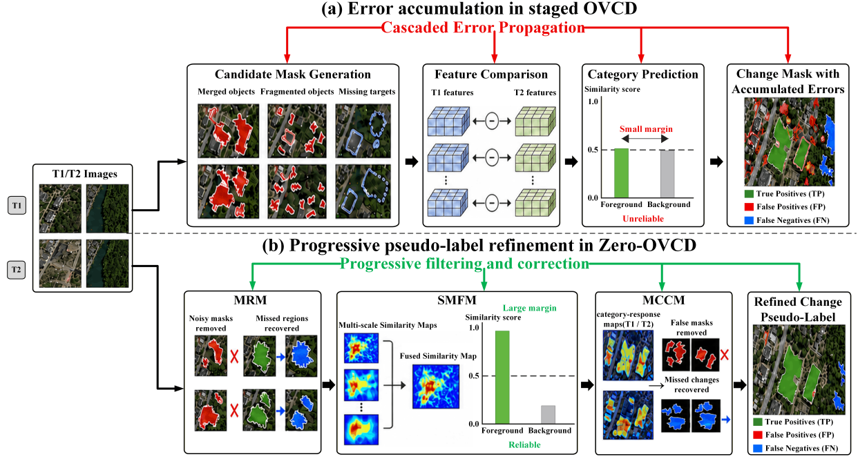
Fig. 1. Schematic comparison between existing staged OVCD and progressive pseudo-label refinement in Zero-OVCD. (a) Candidate-mask defects and ambiguous semantic predictions propagate through staged inference, producing accumulated false positives and false negatives. (b) MRM, SMFM, and MCCM progressively refine candidate masks, improve semantic reliability, and correct incomplete predictions to generate refined pseudo-labels.
