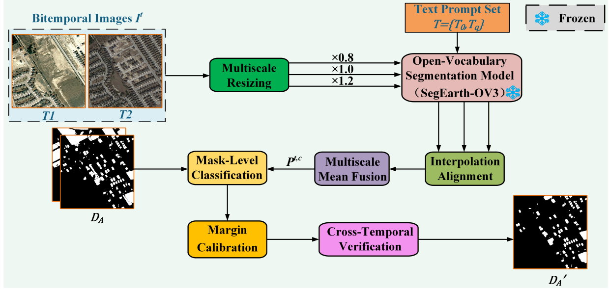
Fig. 4. Illustration of similarity-based multiscale fusion (SMFM). Multiscale category-similarity maps are fused for mask-level classification, followed by background-aware margin filtering and cross-temporal verification to retain reliable change proposals.
