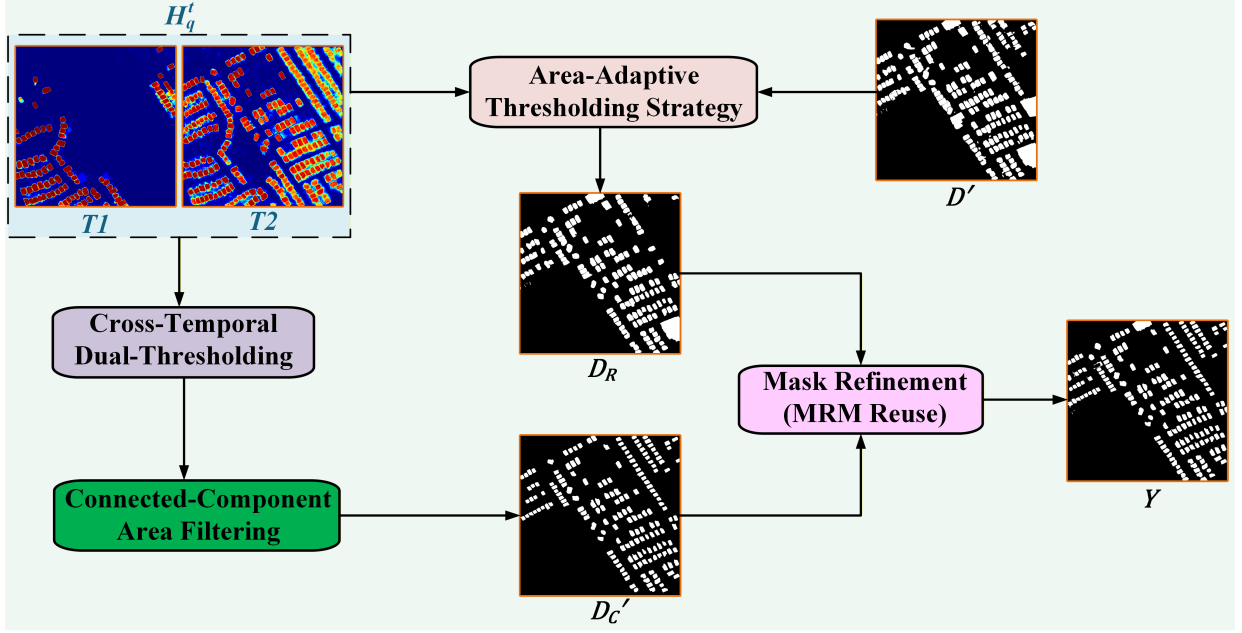
Fig. 5. Illustration of response-guided mask correction and completion (MCCM). Semantic-support filtering removes unreliable proposals, whereas cross-temporal response differences identify changes missed by earlier stages.
