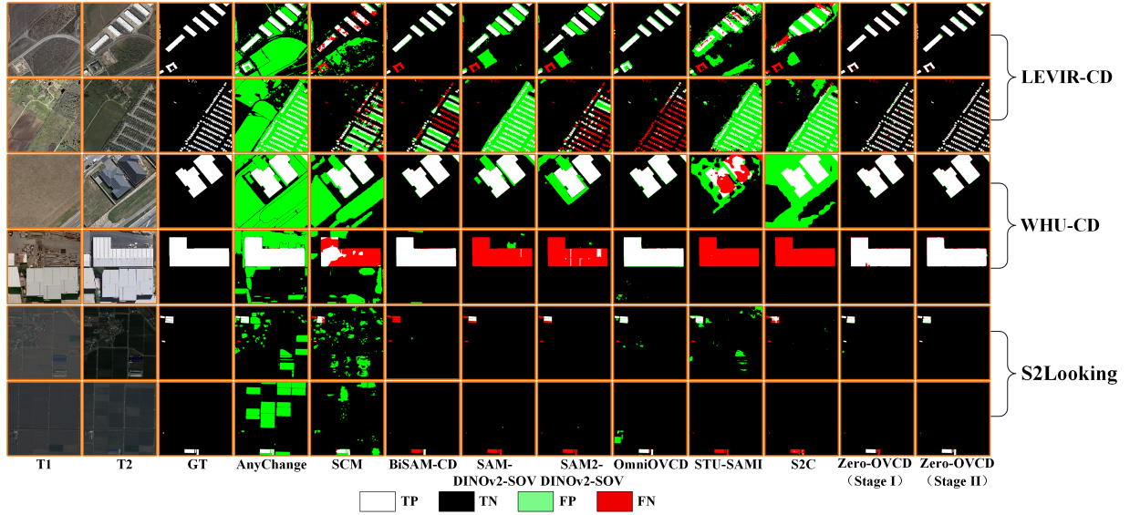
Fig. 7. Qualitative comparison on LEVIR-CD, WHU-CD, and S2Looking. SOV denotes SegEarth-OV.
