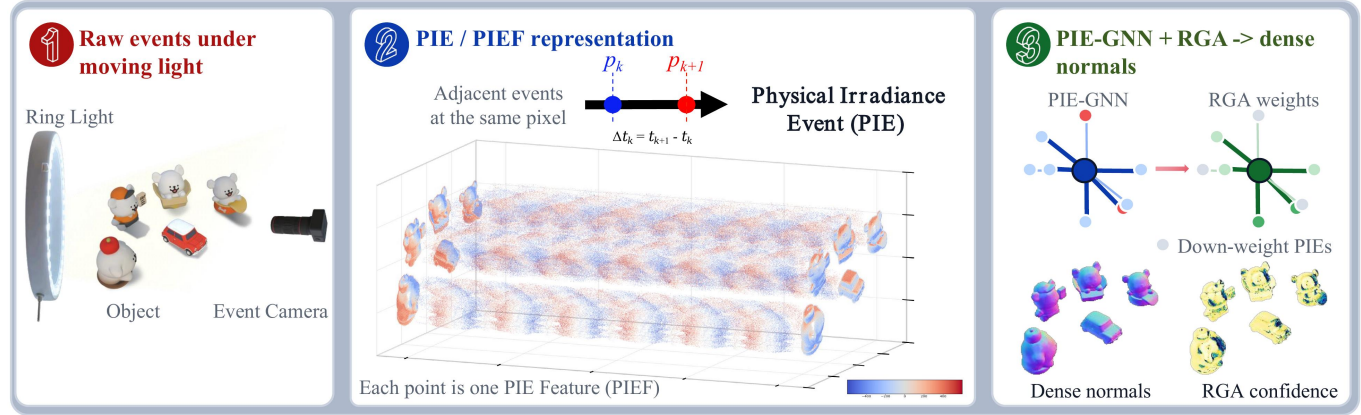
Fig. 1. Overview of PIE-PS. A prototype system captures raw event streams under moving light. Adjacent events at the same pixel are paired with their light directions to form Physical Irradiance Event (PIE) observations. Each PIE provides a threshold-free signed event-rate Physical Irradiance Event Feature (PIEF) and calibrated light-pair geometry. PIE-GNN encodes these PIE nodes, Reliability-Grading Attention (RGA) down-weights unreliable observations, and pixel aggregation produces dense surface normals.
