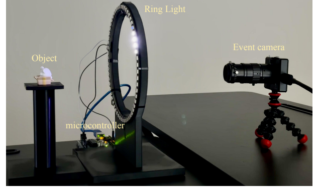
Fig. 4. Prototype acquisition system used for real-world event-based photometric stereo.
