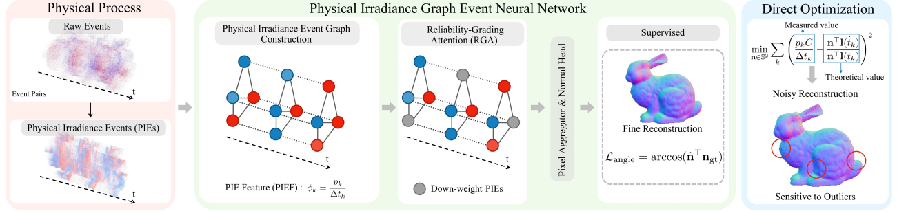
Fig. 2. Overview of the PIE-PS framework. We first convert raw events under moving light into PIE observations. Each PIE provides a threshold-free signed event-rate feature and a corresponding light-pair geometry. The PIE-GNN encodes these observations, uses Reliability-Grading Attention (RGA) to weight them, aggregates pixel features, and predicts normals with a pixel aggregator.
