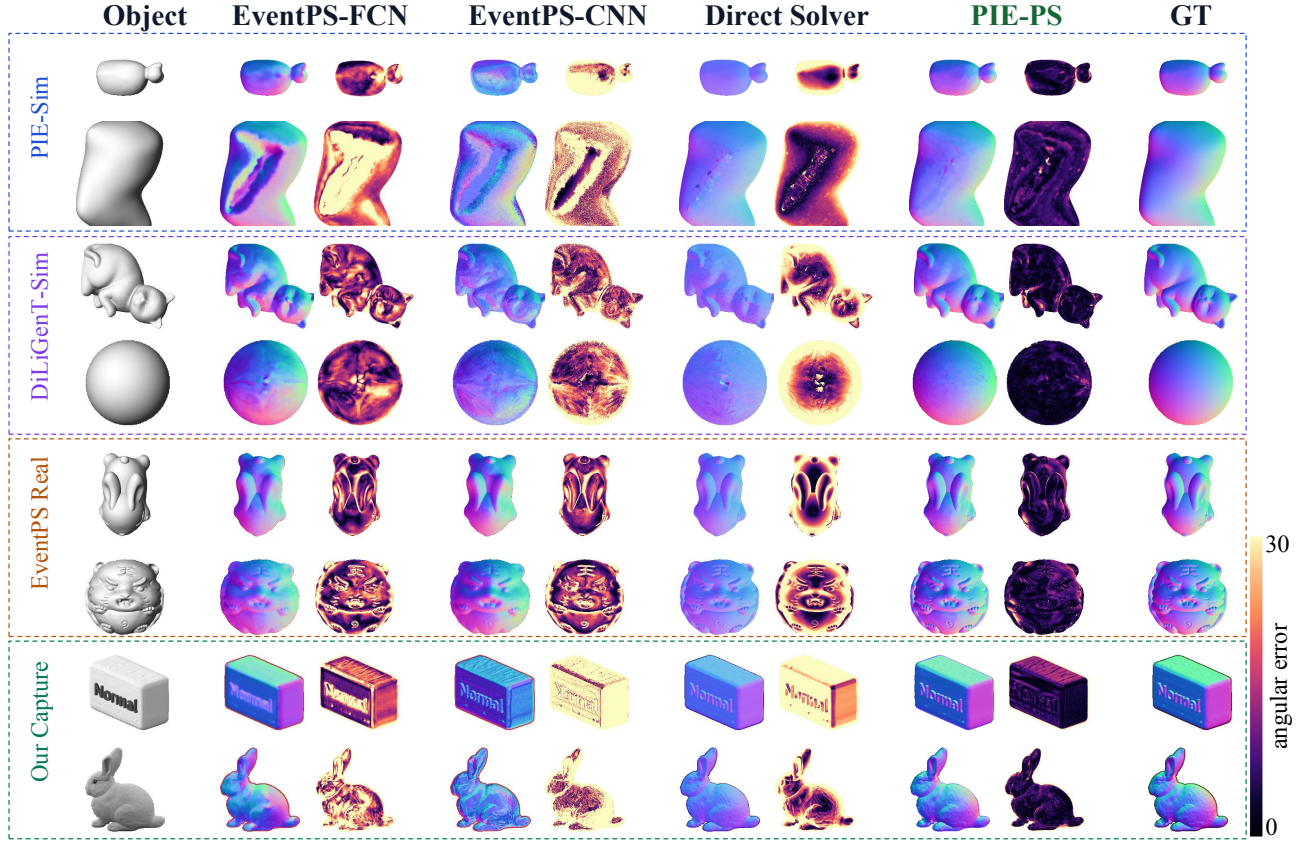
Fig. 5. Qualitative comparison across synthetic and real scenes. Each row shows the object, the normal prediction and angular error map of each method, and the ground-truth normal. We include PIE-Sim, DiLiGenT-Sim, EventPS real scenes, and our captured scenes. Error maps use the same 0^\circ – 30^\circ color range, where darker colors indicate lower error.
