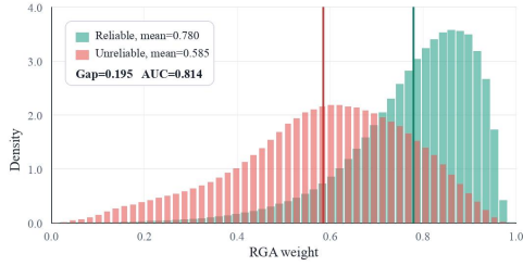
Fig. 7. RGA weight distribution on PIE-Sim. GT-identified unreliable PIEs receive lower weights on average, supporting RGA as a soft reliability-weighting module.
