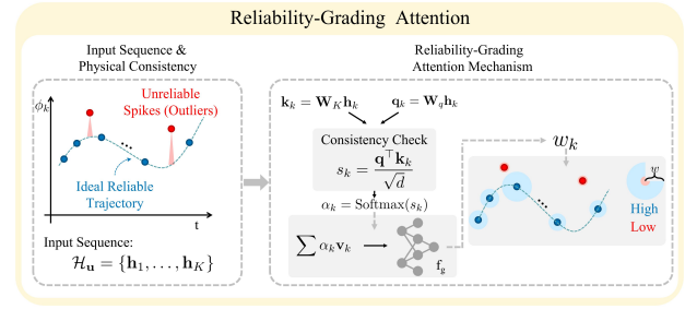
Fig. 3. The Reliability-Grading Attention module scores each event-pair observation. It detects spikes in the PIE sequence and predicts a confidence weight for each observation. The weighted observations are then aggregated into pixel features.
